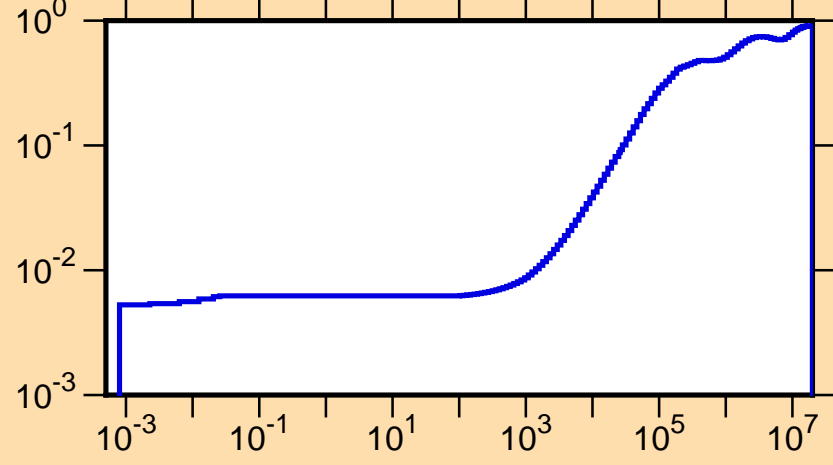
\mu vs. E for ^{129}\text{Pm}(\text{mt251})
