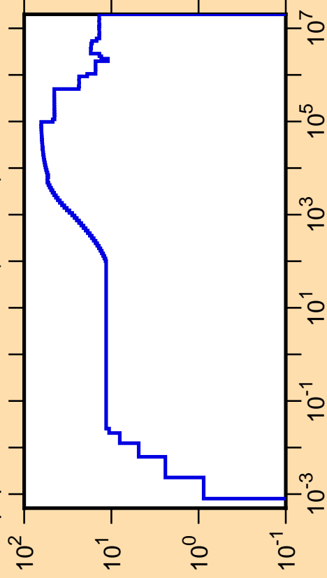
\Delta\mu/\mu vs. E for ^{129}\text{Pm}(\text{mt251})
