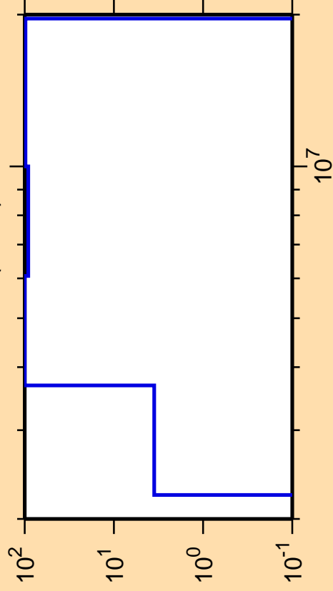
\Delta\sigma/\sigma vs. E for ^{129}\text{Pm}(n,n\alpha)
