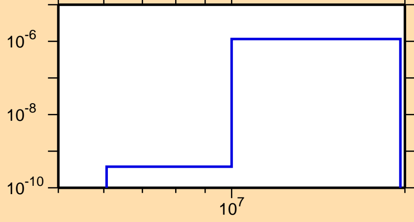
\sigma vs. E for ^{129}\text{Pm}(\text{mt117})
