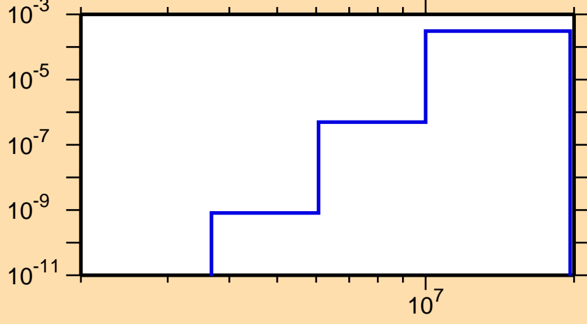
\sigma vs. E for ^{129}\text{Pm}(n,n\alpha)
