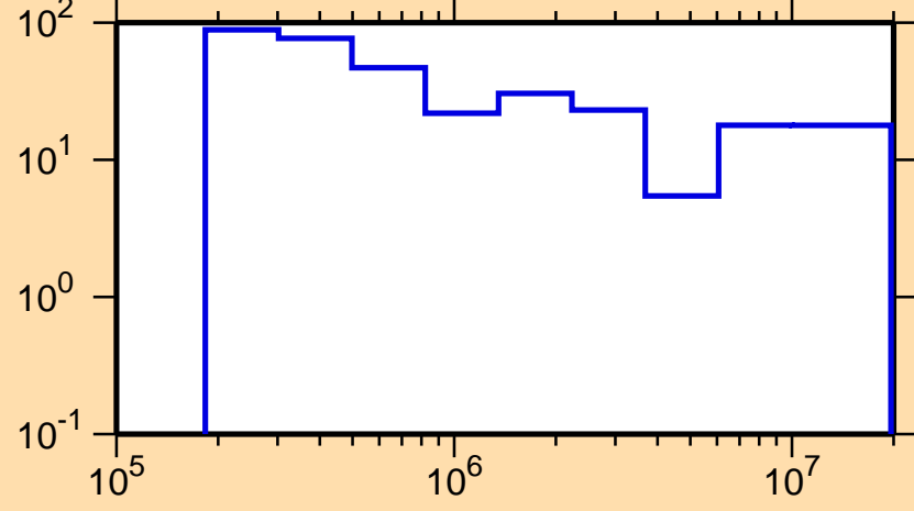
\Delta\sigma/\sigma vs. E for ^{129}\text{Pm}(n,\text{el.})
