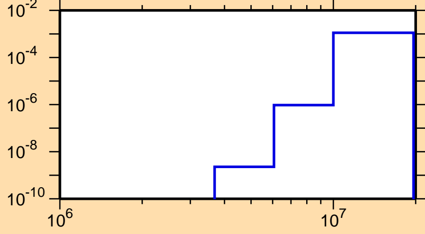
\sigma vs. E for ^{129}\text{Pm}(n,\text{He3})
