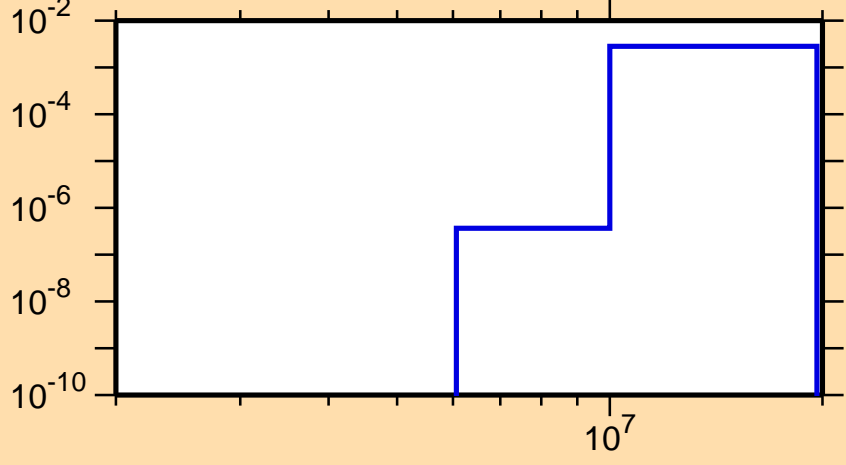
\sigma vs. E for ^{129}\text{Pm}(n,pd)
