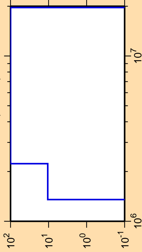
\Delta\sigma/\sigma vs. E for ^{129}\text{Pm}(n,\text{He3})
