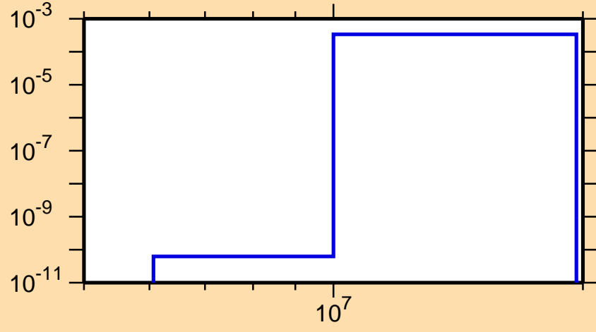
\sigma vs. E for ^{129}\text{Pm}(n,t)
