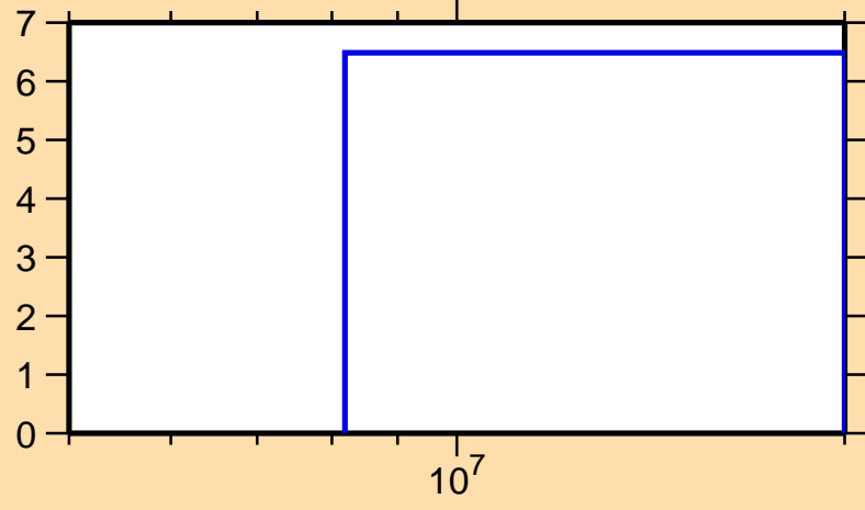
\Delta\sigma/\sigma vs. E for ^{129}\text{Pm}(n,\text{tot.})
