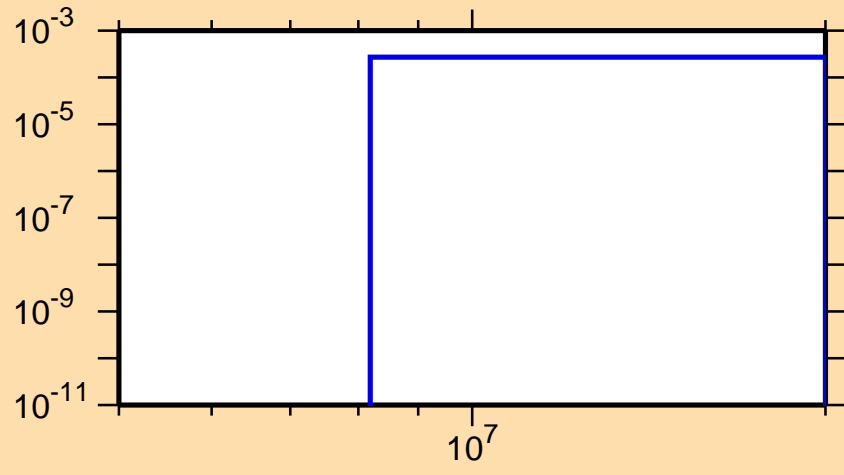
\sigma vs. E for ^{129}\text{Pm}(n,t)
