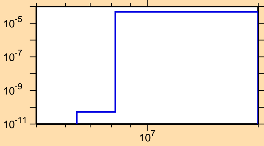
\sigma vs. E for ^{129}\text{Pm}(\text{mt } 45)
