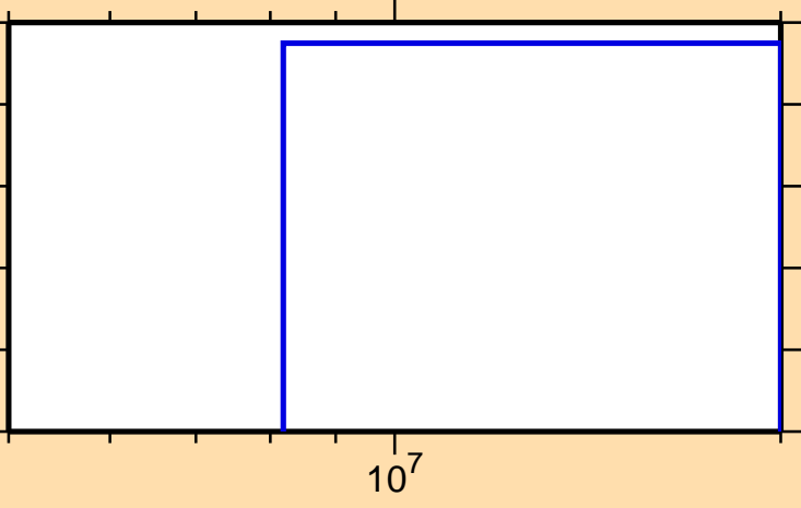
\sigma vs. E for ^{129}\text{Pm}(n,pt)
