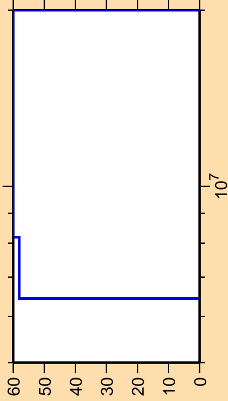
\Delta\sigma/\sigma vs. E for ^{129}\text{Pm}(\text{mt } 45)
