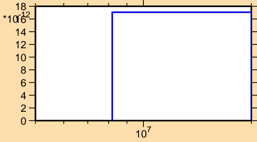
\sigma vs. E for ^{129}\text{Pm}(\text{mt } 34)
