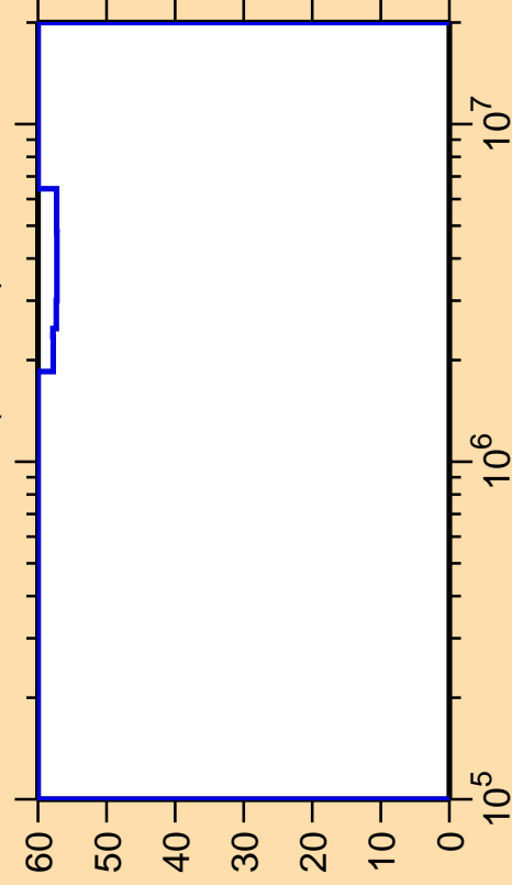
\Delta\sigma/\sigma vs. E for ^{129}\text{Pm}(n,\text{inel.})
