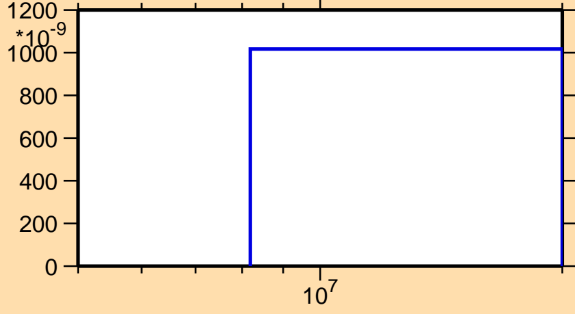
\sigma vs. E for ^{129}\text{Pm}(n,2np)
