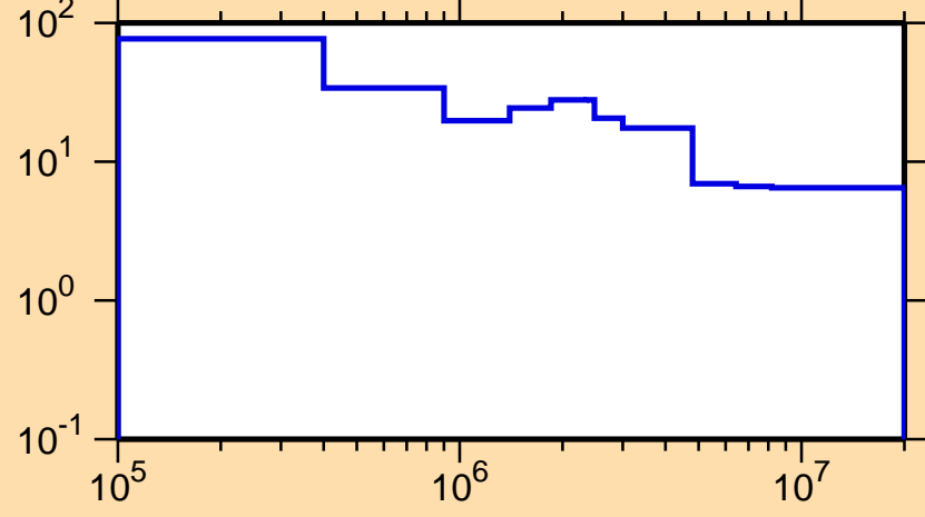
\Delta\sigma/\sigma vs. E for ^{129}\text{Pm}(n,\text{tot.})
