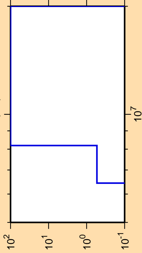
\Delta\sigma/\sigma vs. E for ^{129}\text{Pm}(n,t)
