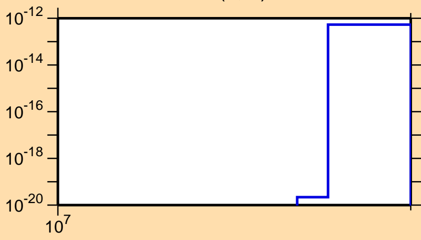
\sigma vs. E for ^{130}\text{Pm}(n,nt)
