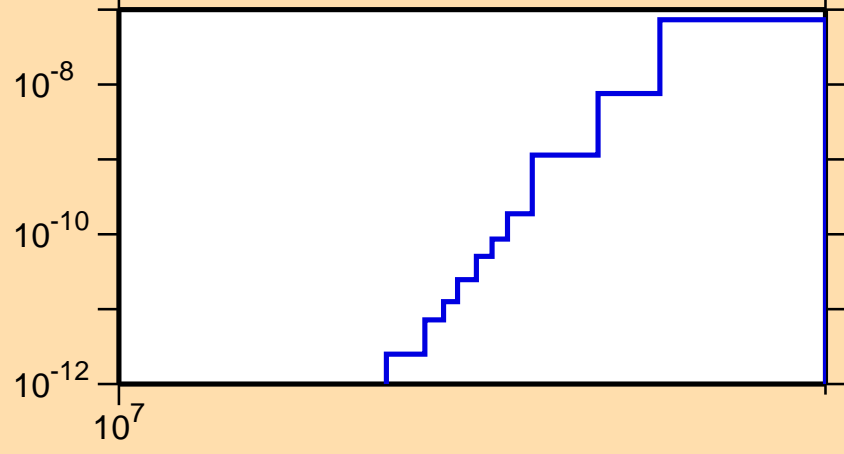
\sigma vs. E for ^{130}\text{Pm} (mt 34)
