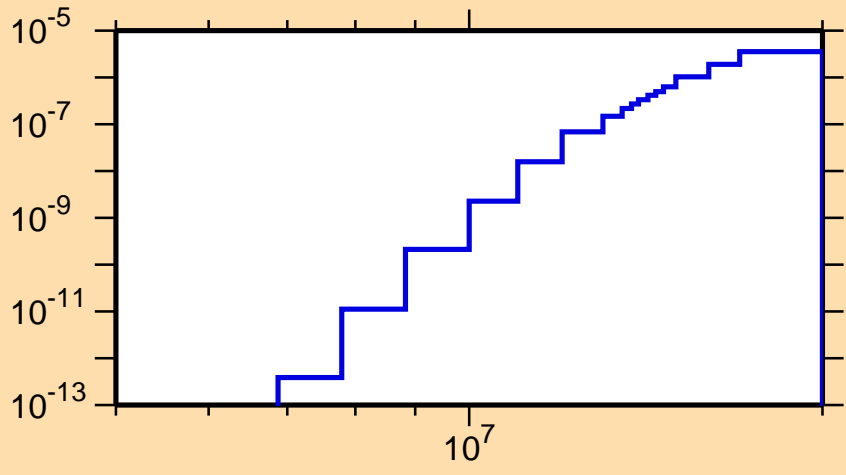
\sigma vs. E for ^{130}\text{Pm}(\text{mt117})
