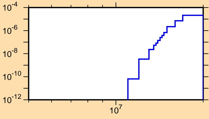
\sigma vs. E for ^{130}\text{Pm}(n,\text{nd})
