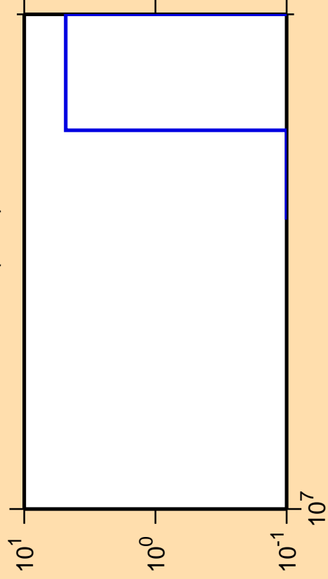
\Delta\sigma/\sigma vs. E for ^{130}\text{Pm}(n,nt)
