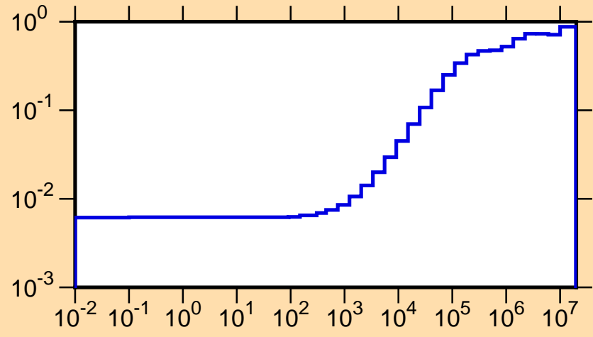
\mu vs. E for ^{130}\text{Pm}(\text{mt251})
