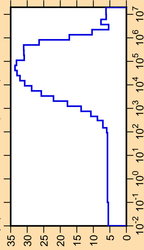
\Delta\mu/\mu vs. E for ^{130}\text{Pm}(\text{mt251})
