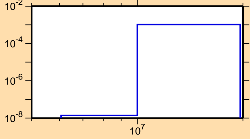
\sigma vs. E for ^{130}\text{Pm}(n,pd)
