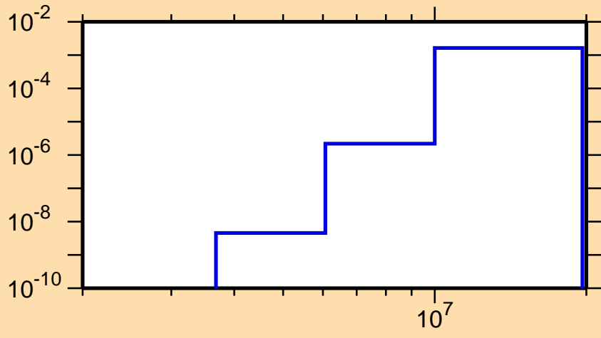
\sigma vs. E for ^{130}\text{Pm}(n,\text{He3})
