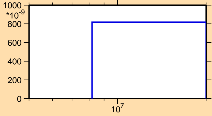
\sigma vs. E for ^{130}\text{Pm}(n,\text{nd})
