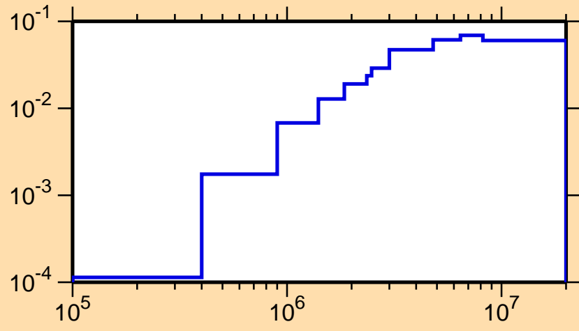
\sigma vs. E for ^{130}\text{Pm}(n,n\text{cont.})
