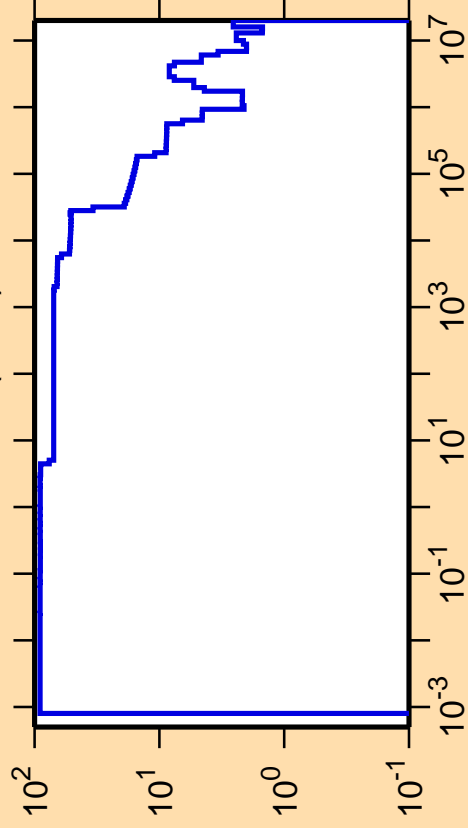
\Delta\sigma/\sigma vs. E for ^{131}\text{Pm}(n,\text{el.})
