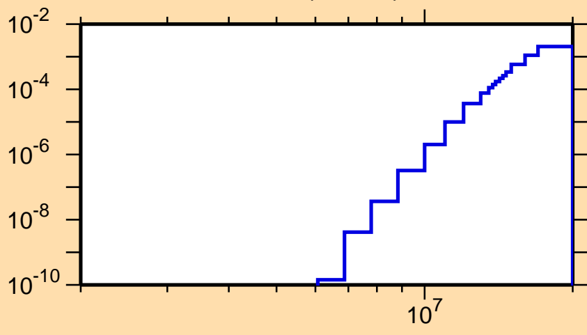
\sigma vs. E for ^{131}\text{Pm}(n,\text{He}3)
