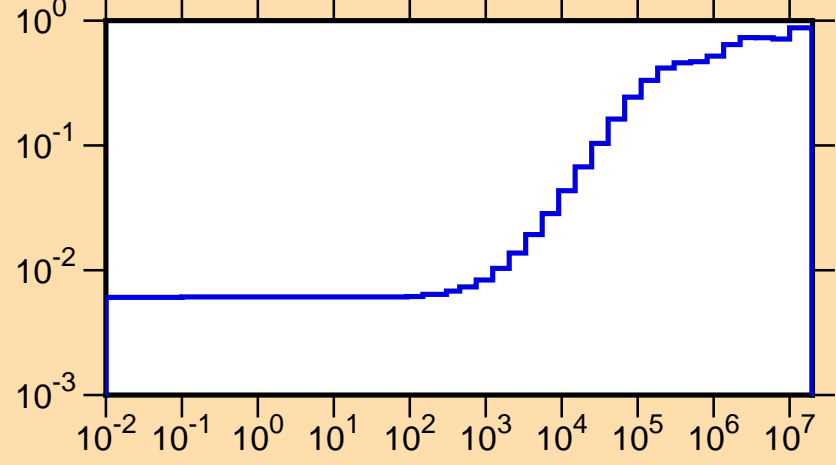
\mu vs. E for ^{131}\text{Pm}(\text{mt251})
