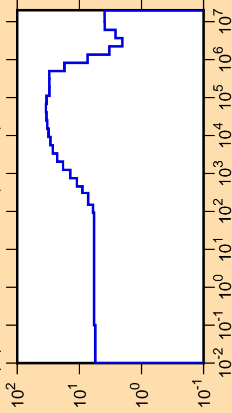
\Delta\mu/\mu vs. E for ^{131}\text{Pm}(\text{mt251})
