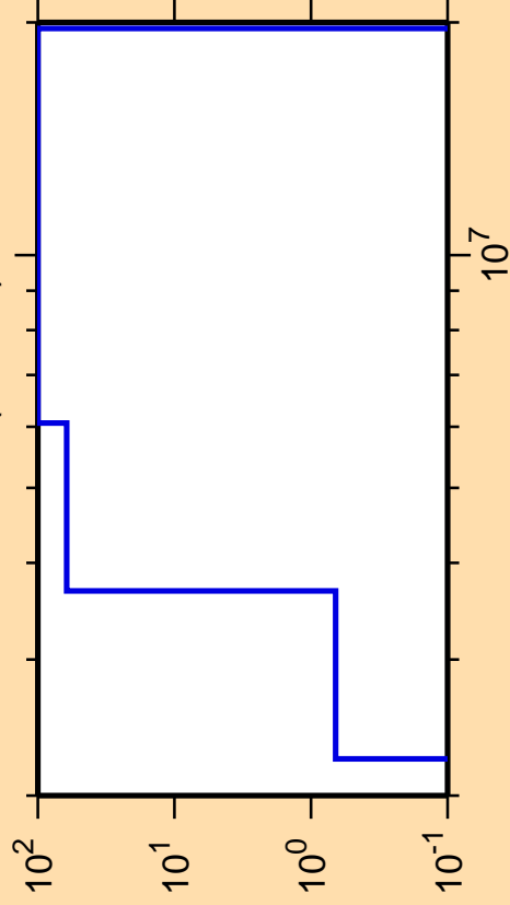
\Delta\sigma/\sigma vs. E for ^{131}\text{Pm}(n,\text{He3})
