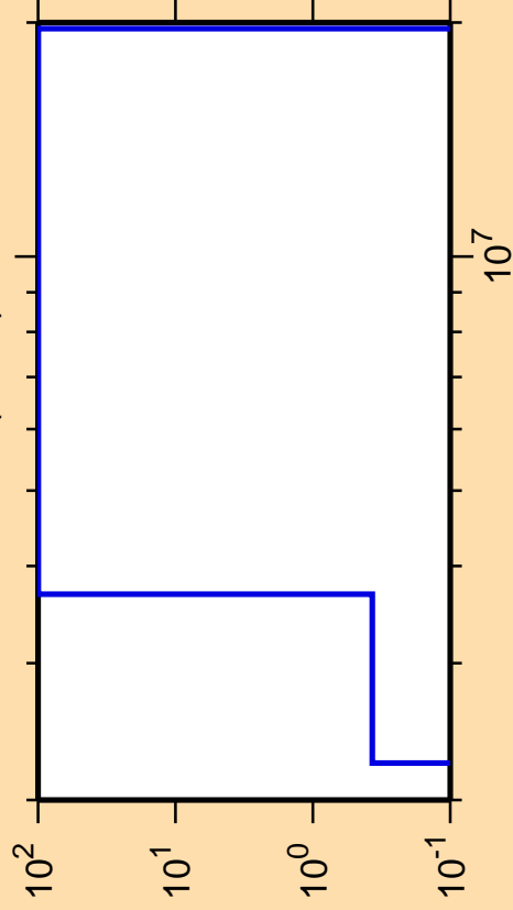
\Delta\sigma/\sigma vs. E for ^{131}\text{Pm}(n,n\alpha)
