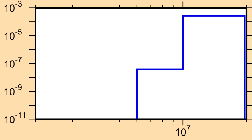
\sigma vs. E for ^{131}\text{Pm}(n,\text{He3})
