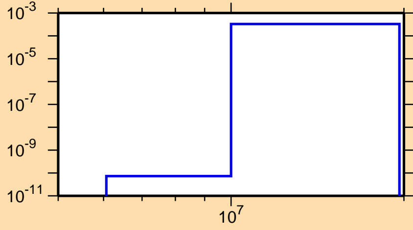
\sigma vs. E for ^{131}\text{Pm}(n,t)
