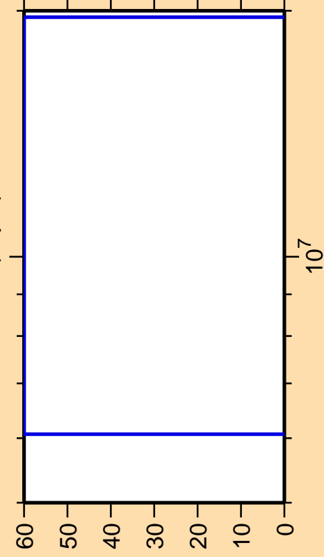
\Delta\sigma/\sigma vs. E for ^{131}\text{Pm}(n,\text{pd})
