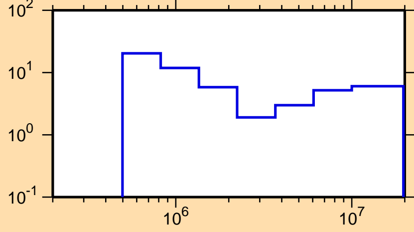
\Delta\sigma/\sigma vs. E for ^{131}\text{Pm}(n,\text{nonel.})
