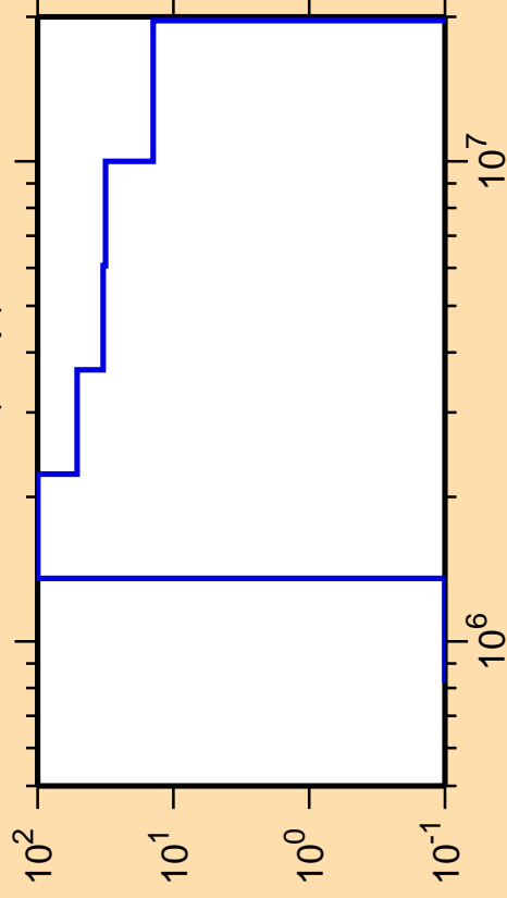
\Delta\sigma/\sigma vs. E for ^{131}\text{Pm}(n,np)
