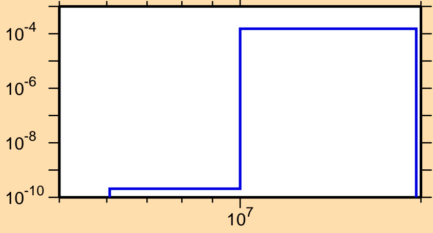
\sigma vs. E for ^{131}\text{Pm}(n,\text{pd})
