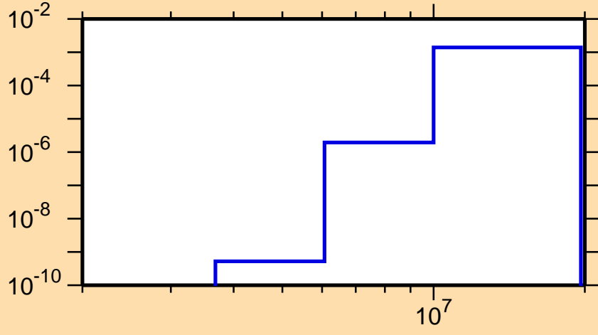
\sigma vs. E for ^{131}\text{Pm}(n,n\alpha)
