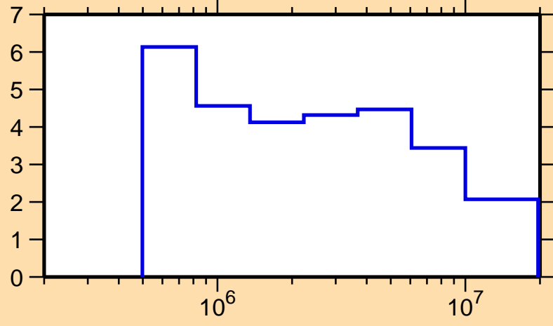
\Delta\sigma/\sigma vs. E for ^{131}\text{Pm}(n,\text{tot.})
