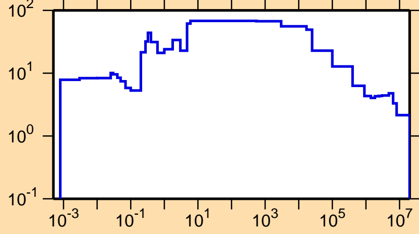
\Delta\sigma/\sigma vs. E for ^{131}\text{Pm}(n,\text{tot.})
