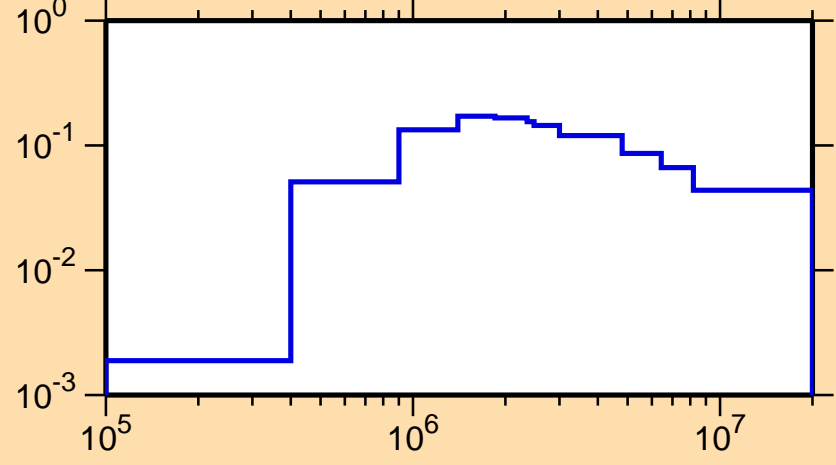
\sigma vs. E for ^{131}\text{Pm}(n,\text{inel.})
