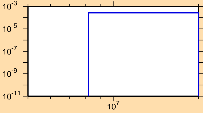
\sigma vs. E for ^{131}\text{Pm}(n,t)
