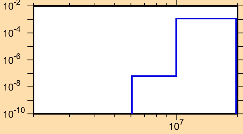
\sigma vs. E for ^{132}\text{Pm}(n,t)
