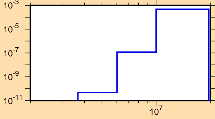
\sigma vs. E for ^{132}\text{Pm}(n,\text{He3})
