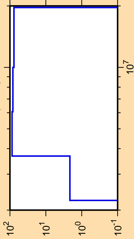
\Delta\sigma/\sigma vs. E for ^{132}\text{Pm}(n,n\alpha)
