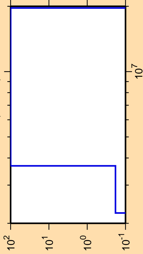
\Delta\sigma/\sigma vs. E for ^{132}\text{Pm}(n,\text{He3})
