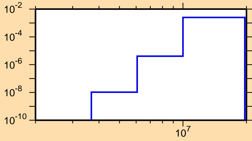
\sigma vs. E for ^{132}\text{Pm}(n,n\alpha)
