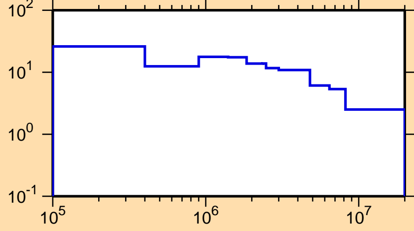
\Delta\sigma/\sigma vs. E for ^{132}\text{Pm}(n,\text{nonel.})
