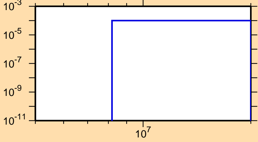
\sigma vs. E for ^{132}\text{Pm}(n,pd)
