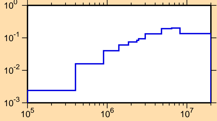
\sigma vs. E for ^{132}\text{Pm}(n,\text{inel.})
