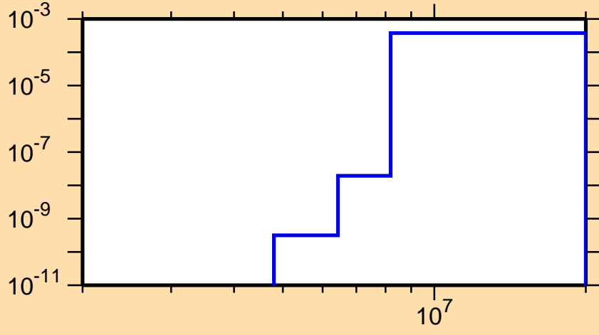
\sigma vs. E for ^{132}\text{Pm}(n,\text{He3})
