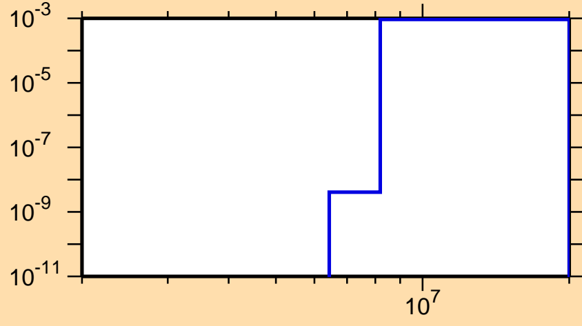
\sigma vs. E for ^{132}\text{Pm}(n,t)
