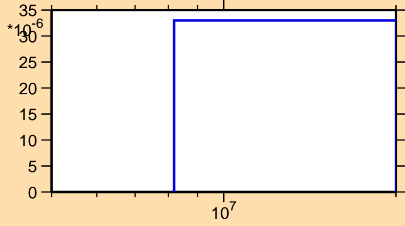
\sigma vs. E for ^{132}\text{Pm}(\text{mt } 45)
