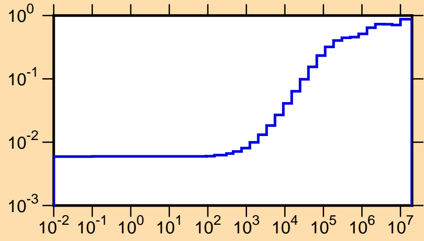
\mu vs. E for ^{133}\text{Pm}(\text{mt251})
