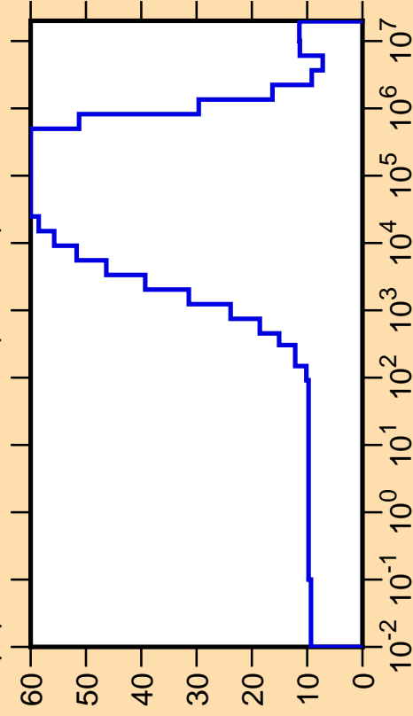
\Delta\mu/\mu vs. E for ^{133}\text{Pm}(\text{mt251})
