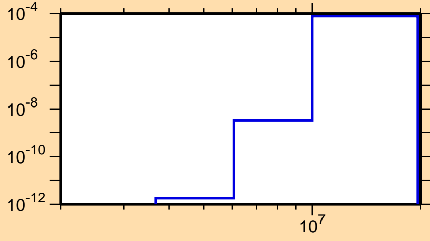
\sigma vs. E for ^{133}\text{Pm}(n,\text{He3})
