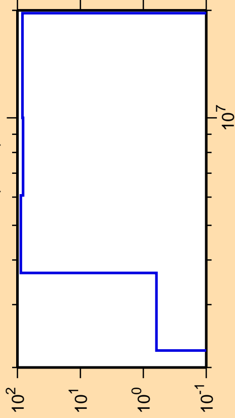
\Delta\sigma/\sigma vs. E for ^{133}\text{Pm}(n,n\alpha)
