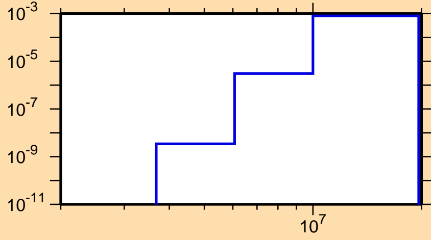
\sigma vs. E for ^{133}\text{Pm}(n,n\alpha)
