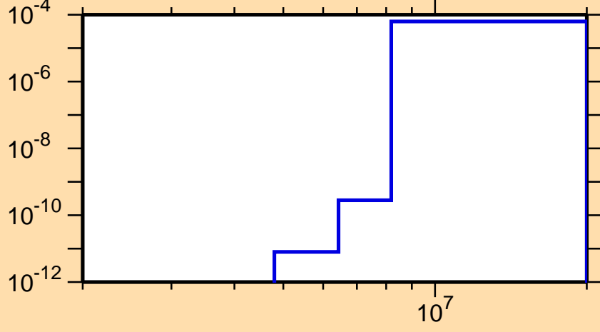
\sigma vs. E for ^{133}\text{Pm}(n,\text{He3})
