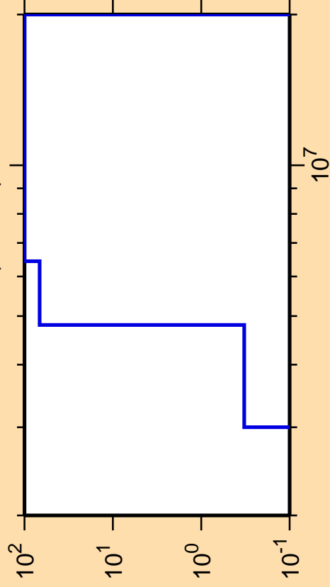
\Delta\sigma/\sigma vs. E for ^{133}\text{Pm}(n,\text{He3})
