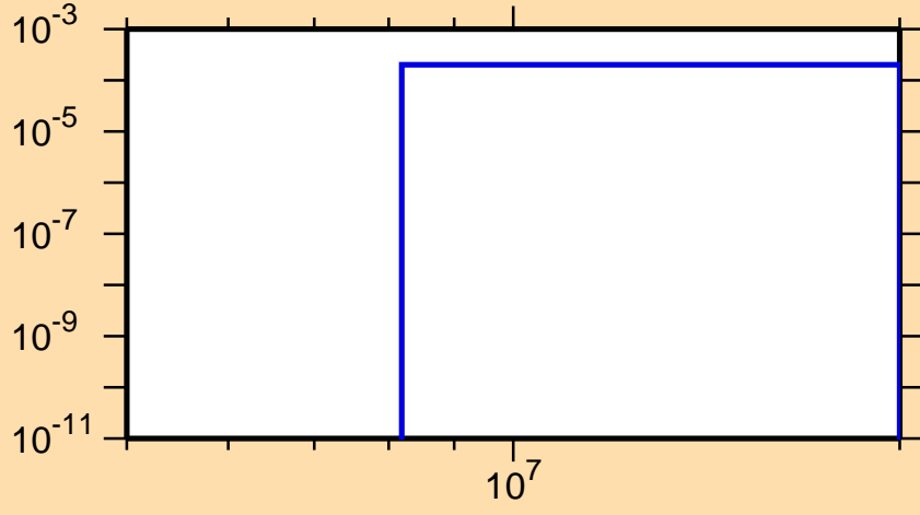
\sigma vs. E for ^{133}\text{Pm}(n,t)
