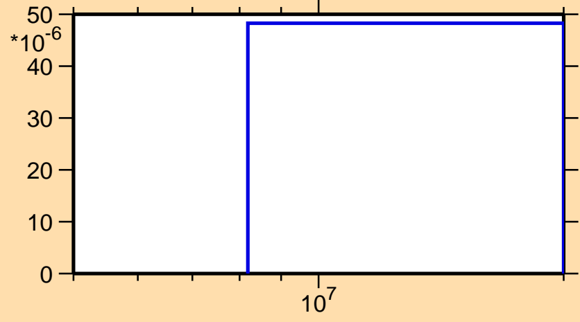
\sigma vs. E for ^{133}\text{Pm}(n,\text{pd})
