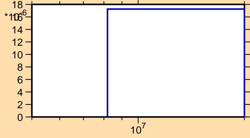
\sigma vs. E for ^{133}\text{Pm}(n,2np)
