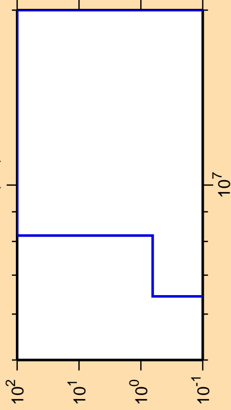
\Delta\sigma/\sigma vs. E for ^{133}\text{Pm}(n,t)
