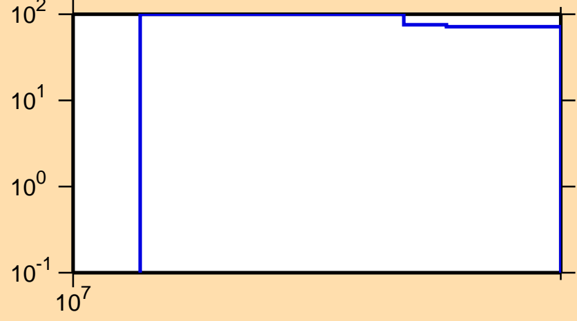
\Delta\sigma/\sigma vs. E for ^{133}\text{Pm}(n,2n)
