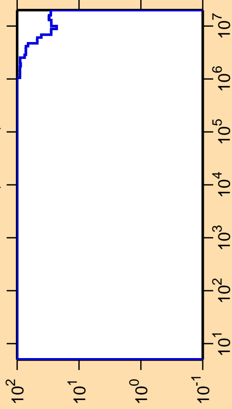
\Delta\sigma/\sigma vs. E for ^{133}\text{Pm}(n,\text{inel.})
