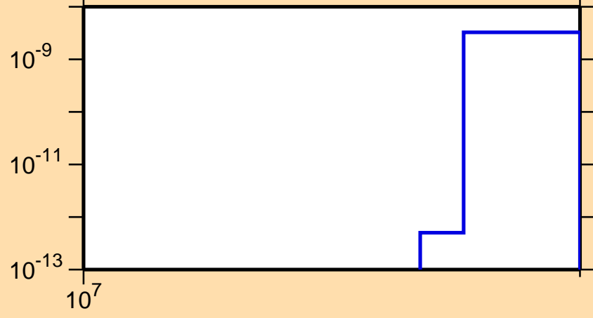
\sigma vs. E for ^{133}\text{Pm}(n,nt)
