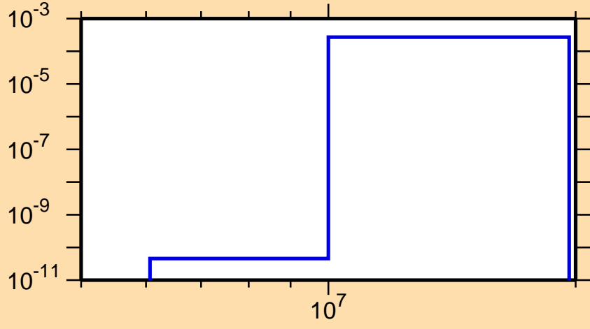
\sigma vs. E for ^{133}\text{Pm}(n,t)
