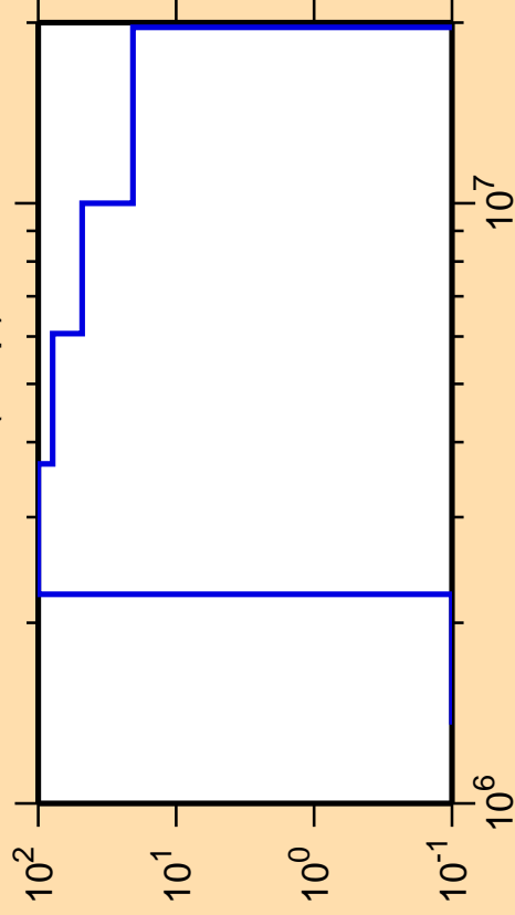
\Delta\sigma/\sigma vs. E for ^{133}\text{Pm}(n,np)
