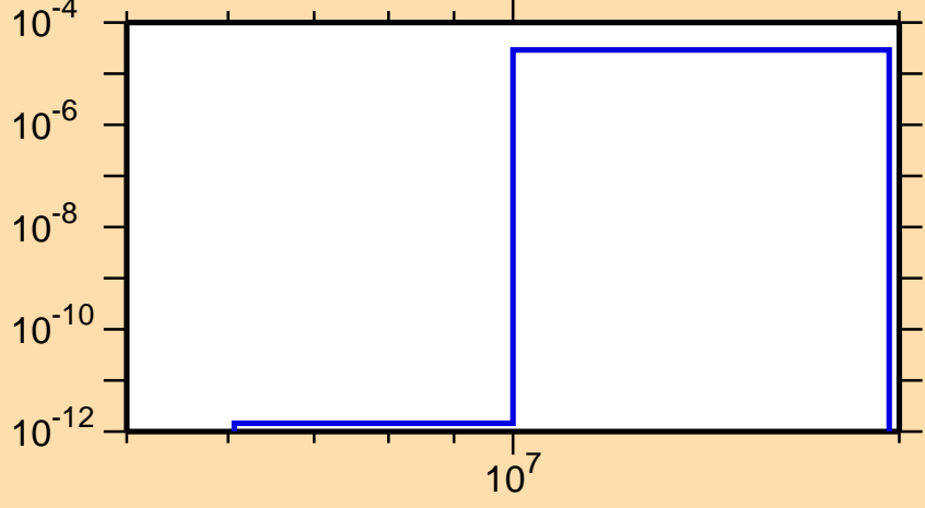
\sigma vs. E for ^{133}\text{Pm}(n,pd)
