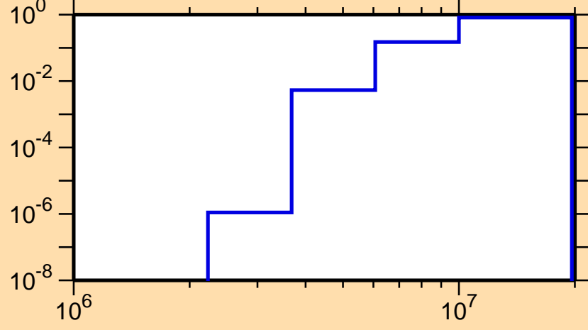
\sigma vs. E for ^{133}\text{Pm}(n,np)
