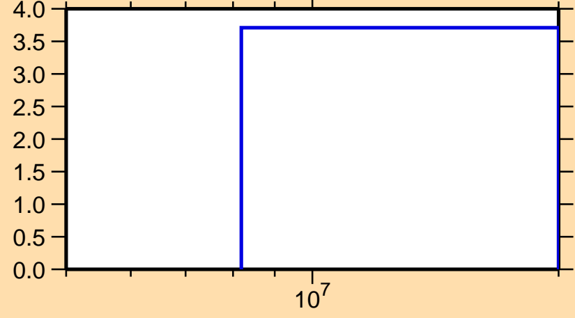
\Delta\sigma/\sigma vs. E for ^{133}\text{Pm}(n,\text{nonel.})
