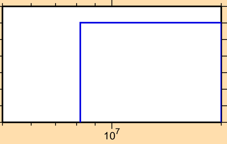
\sigma vs. E for ^{134}\text{Pm}(n,2np)
