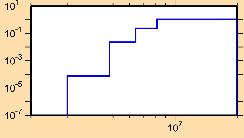
\sigma vs. E for ^{134}\text{Pm}(n,np)
