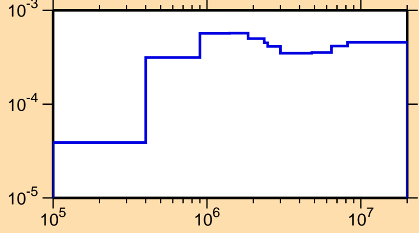
\sigma vs. E for ^{134}\text{Pm}(n,n_2)
