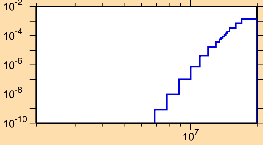
\sigma vs. E for ^{134}\text{Pm}(n,\text{He}3)
