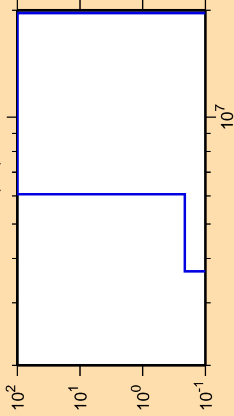
\Delta\sigma/\sigma vs. E for ^{134}\text{Pm}(n,t)
