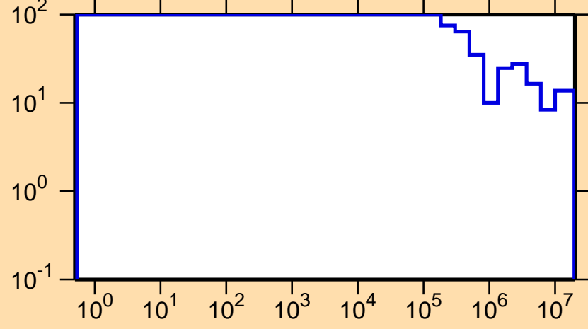
\Delta\sigma/\sigma vs. E for ^{134}\text{Pm}(n,\text{el.})
