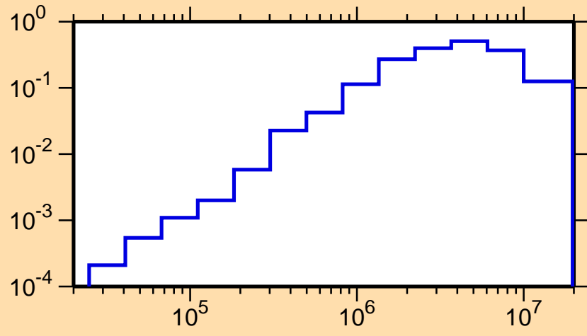
\sigma vs. E for ^{134}\text{Pm}(n,n\text{cont.})
