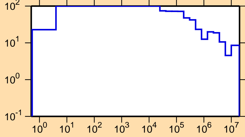
\Delta\sigma/\sigma vs. E for ^{134}\text{Pm}(n,\text{tot.})
