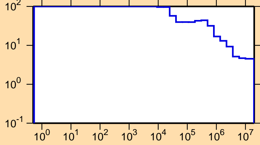
\Delta\sigma/\sigma vs. E for ^{134}\text{Pm}(n,\text{nonel.})
