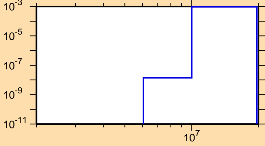
\sigma vs. E for ^{134}\text{Pm}(n,t)
