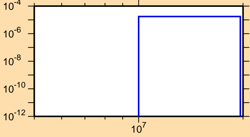
\sigma vs. E for ^{134}\text{Pm}(n,nd)
