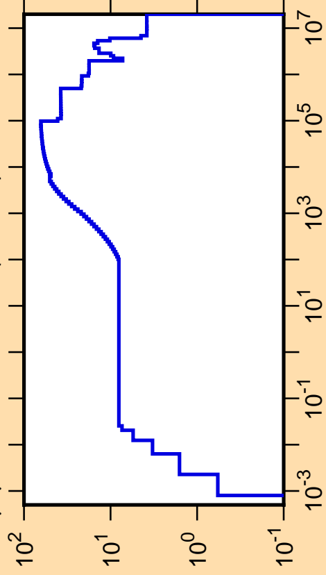
\Delta\mu/\mu vs. E for ^{135}\text{Pm}(\text{mt251})
