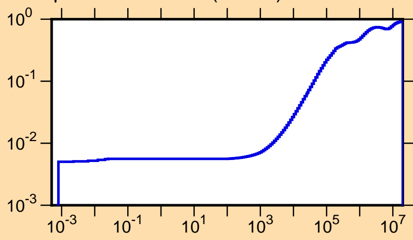
\mu vs. E for ^{135}\text{Pm}(\text{mt251})
