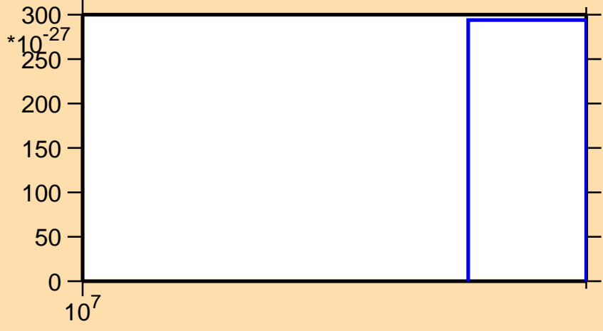
\sigma vs. E for ^{135}\text{Pm}(\text{mt } 11)
