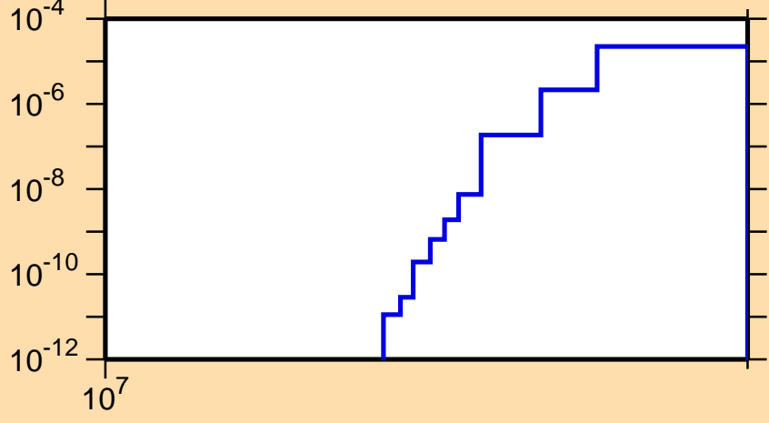
\sigma vs. E for ^{135}\text{Pm}(n,nd)
