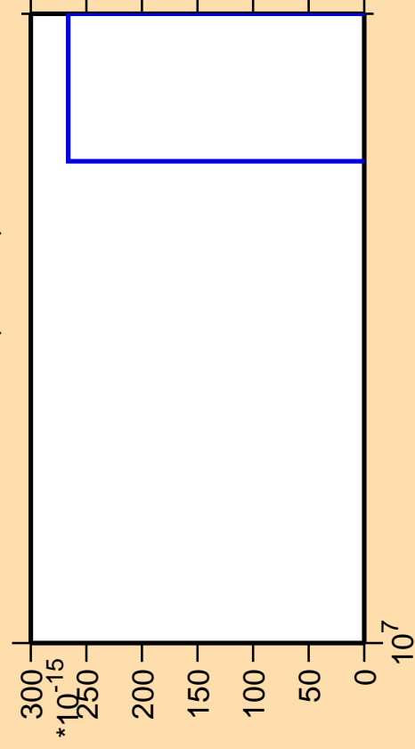
\Delta\sigma/\sigma vs. E for ^{135}\text{Pm}(\text{mt } 11)
