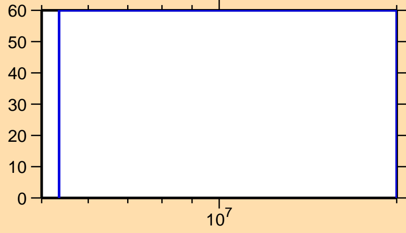
\Delta\sigma/\sigma vs. E for ^{135}\text{Pm}(n,ncont.)
