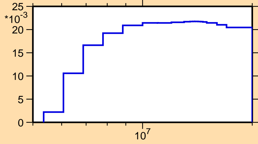
\sigma vs. E for ^{135}\text{Pm}(n,n_2)
