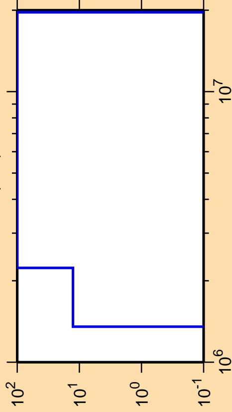
\Delta\sigma/\sigma vs. E for ^{135}\text{Pm}(n,d)
