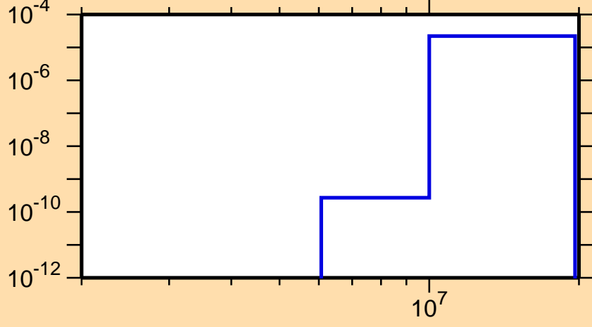
\sigma vs. E for ^{135}\text{Pm}(n,\text{He3})
