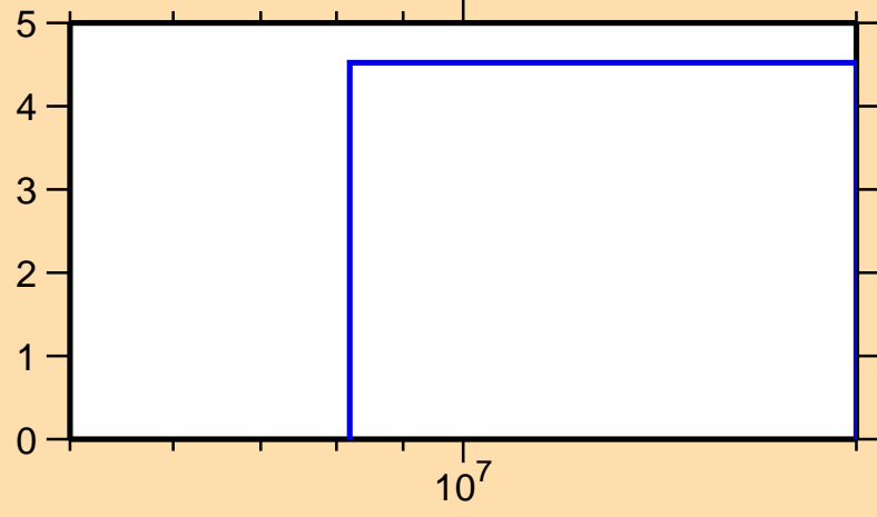
\Delta\sigma/\sigma vs. E for ^{135}\text{Pm}(n,\text{el.})
