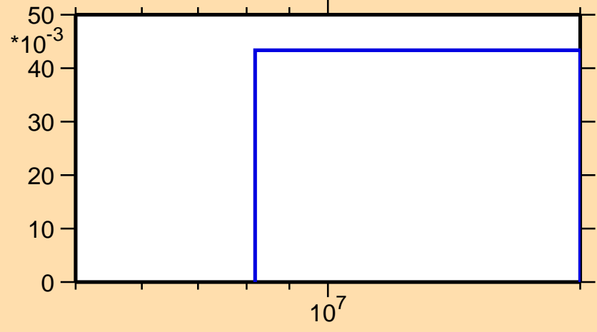
\sigma vs. E for ^{135}\text{Pm}(n,2n)
