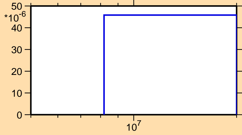
\sigma vs. E for ^{135}\text{Pm}(n,2np)
