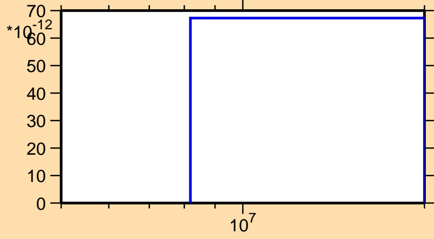
\sigma vs. E for ^{135}\text{Pm}(n,nt)
