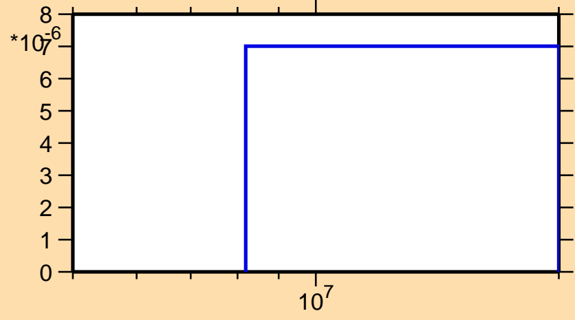
\sigma vs. E for ^{135}\text{Pm}(n,\text{pd})
