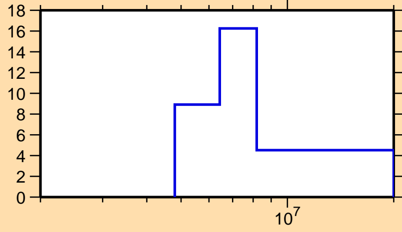
\Delta\sigma/\sigma vs. E for ^{135}\text{Pm}(n,\text{el.})
