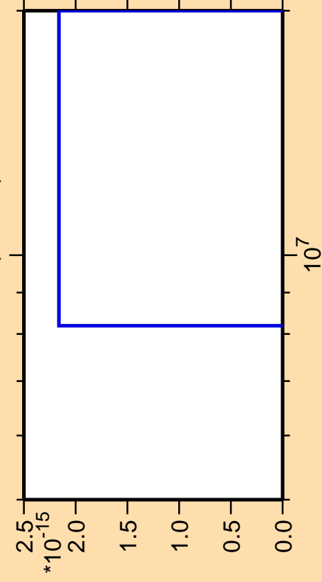
\Delta\sigma/\sigma vs. E for ^{135}\text{Pm} (mt 11)
