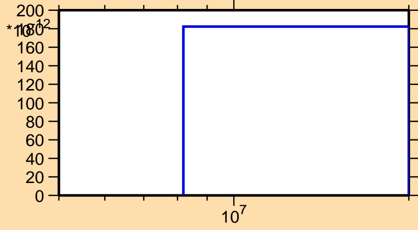
\sigma vs. E for ^{135}\text{Pm}(n,2n\alpha)
