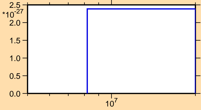
\sigma vs. E for ^{135}\text{Pm} (mt 11)
