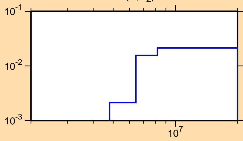
\sigma vs. E for ^{135}\text{Pm}(n,n_2)
