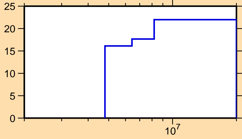
\Delta\sigma/\sigma vs. E for ^{135}\text{Pm}(n,n_1)
