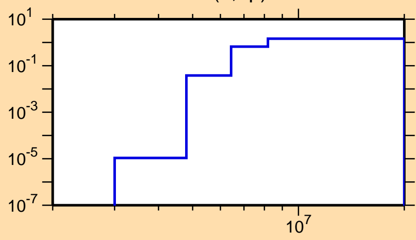
\sigma vs. E for ^{135}\text{Pm}(n,np)
