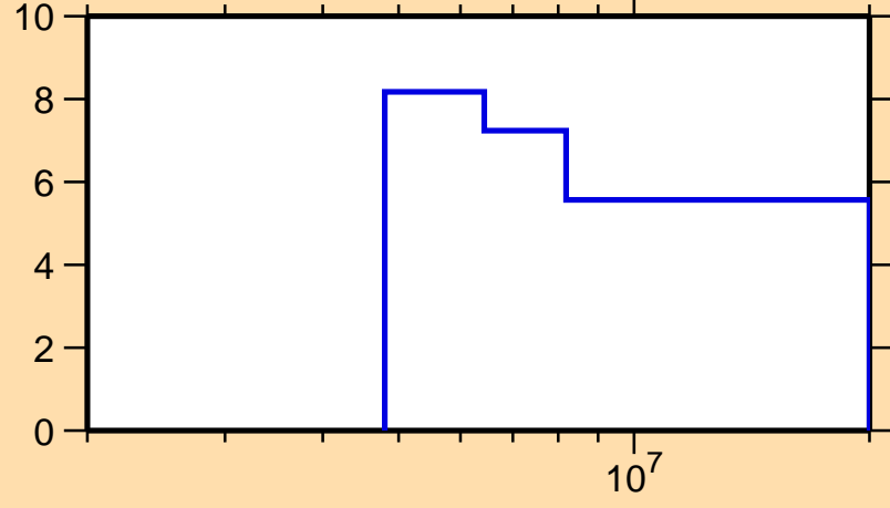
\Delta\sigma/\sigma vs. E for ^{135}\text{Pm}(n,\text{nonel.})
