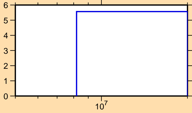
\Delta\sigma/\sigma vs. E for ^{135}\text{Pm}(n,\text{nonel.})
