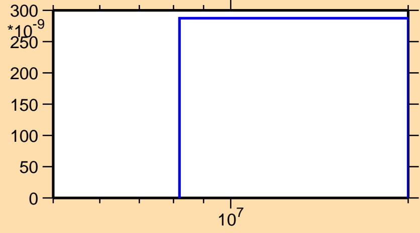
\sigma vs. E for ^{135}\text{Pm}(n,\text{nd})
