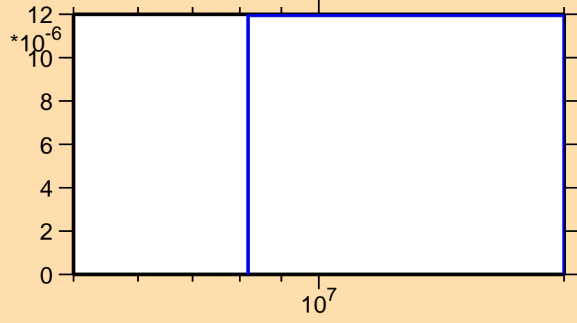
\sigma vs. E for ^{135}\text{Pm}(\text{mt 45})
