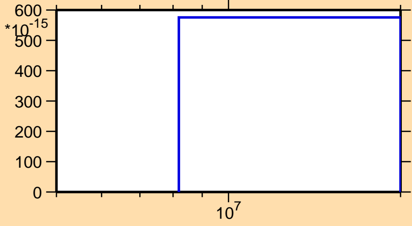
\sigma vs. E for ^{135}\text{Pm} (mt 34)
