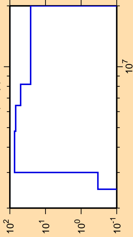
\Delta\sigma/\sigma vs. E for ^{135}\text{Pm}(n,np)
