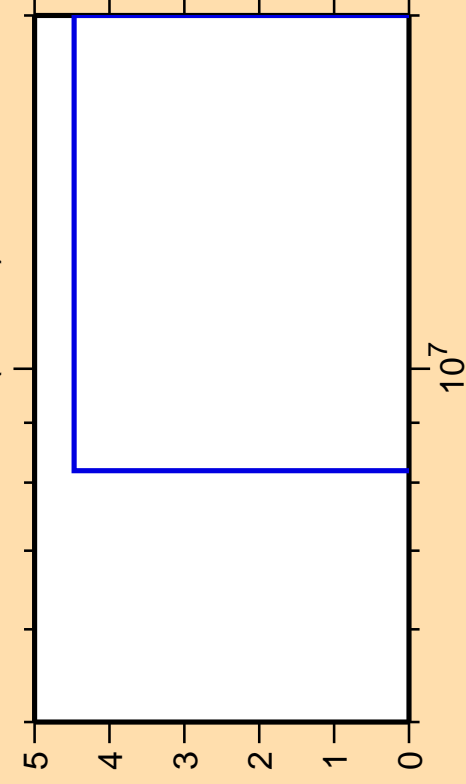
\Delta\sigma/\sigma vs. E for ^{135}\text{Pm} (mt 34)
