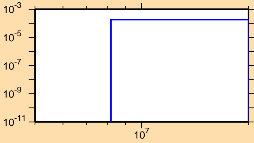
\sigma vs. E for ^{135}\text{Pm}(n,t)
