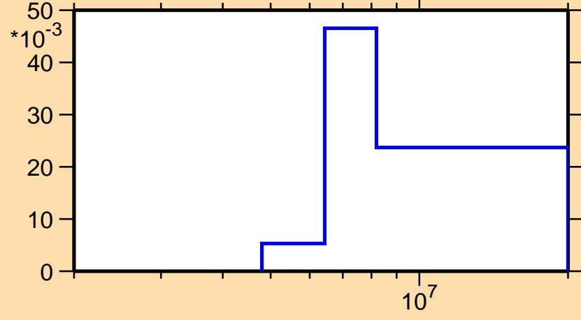
\sigma vs. E for ^{135}\text{Pm}(n,n\text{cont.})
