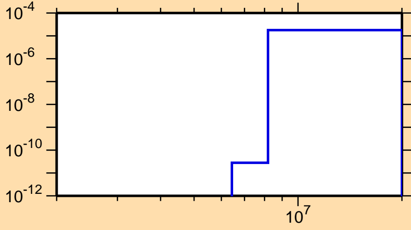
\sigma vs. E for ^{135}\text{Pm}(n,\text{He3})
