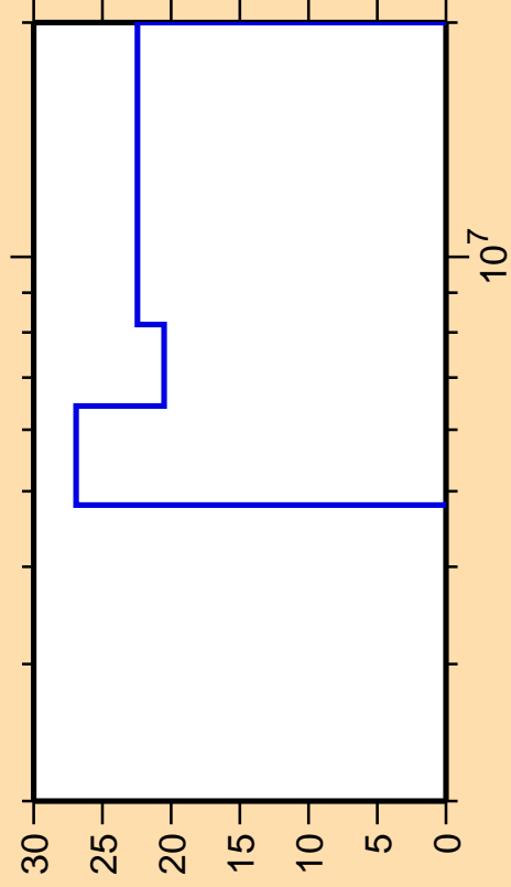
\Delta\sigma/\sigma vs. E for ^{135}\text{Pm}(n,n_2)
