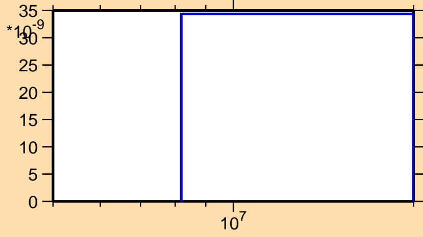
\sigma vs. E for ^{135}\text{Pm}(\text{mt117})
