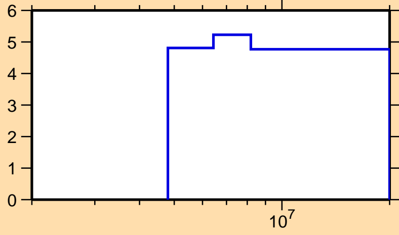
\Delta\sigma/\sigma vs. E for ^{135}\text{Pm}(n,\text{tot.})
