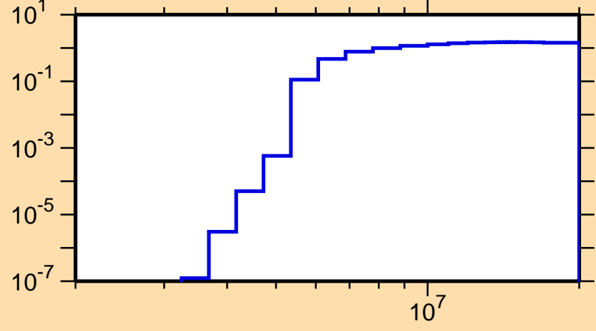
\sigma vs. E for ^{135}\text{Pm}(n,np)
