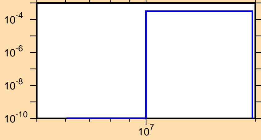
\sigma vs. E for ^{135}\text{Pm}(n,t)
