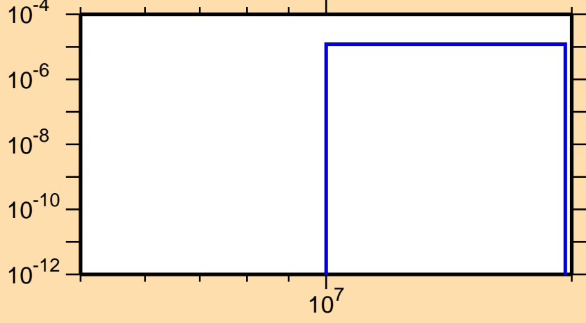
\sigma vs. E for ^{135}\text{Pm} (mt 45)
