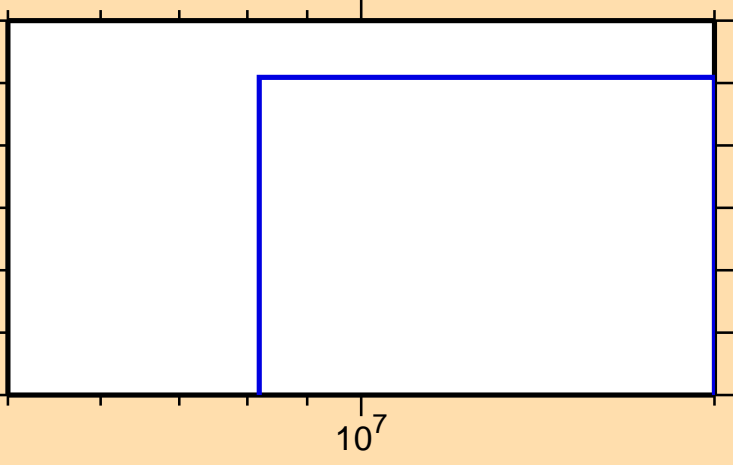
\sigma vs. E for ^{135}\text{Pm}(\text{mt117})
