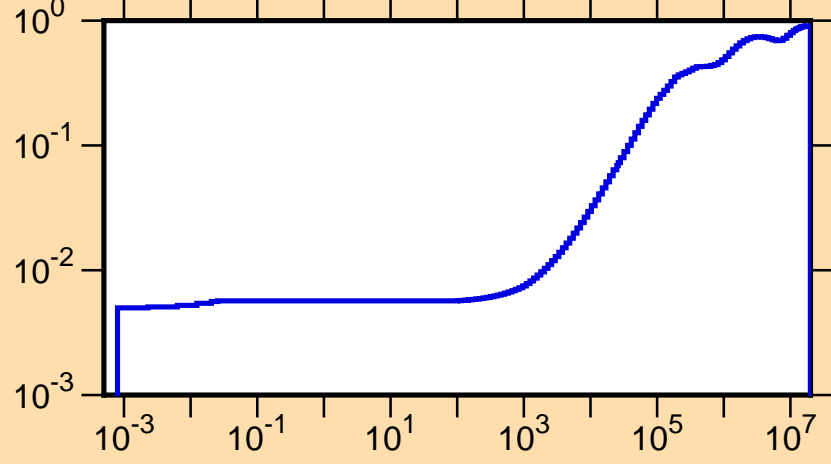
\mu vs. E for ^{136}\text{Pm}(\text{mt251})
