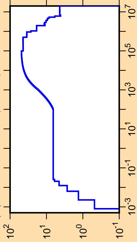
\Delta\mu/\mu vs. E for ^{136}\text{Pm}(\text{mt251})
