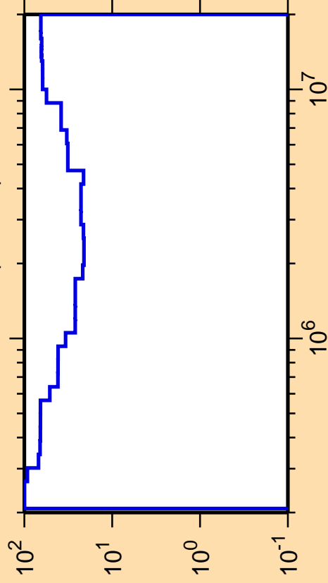
\Delta\sigma/\sigma vs. E for ^{136}\text{Pm}(n,\text{inel.})
