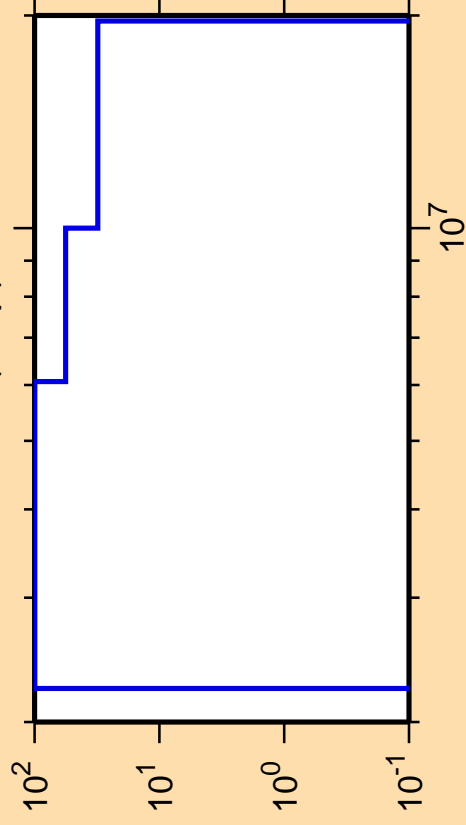
\Delta\sigma/\sigma vs. E for ^{136}\text{Pm}(n,np)
