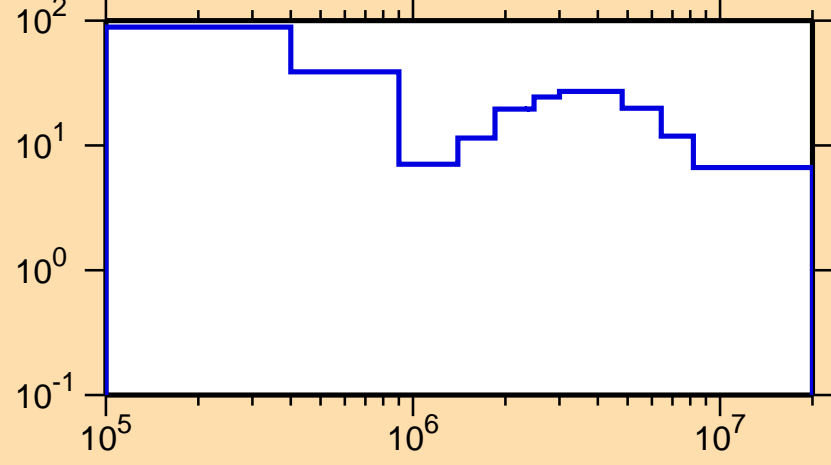
\Delta\sigma/\sigma vs. E for ^{136}\text{Pm}(n,\text{el.})
