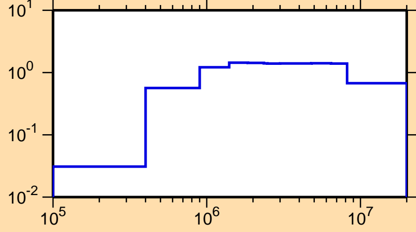
\sigma vs. E for ^{136}\text{Pm}(n,\text{inel.})
