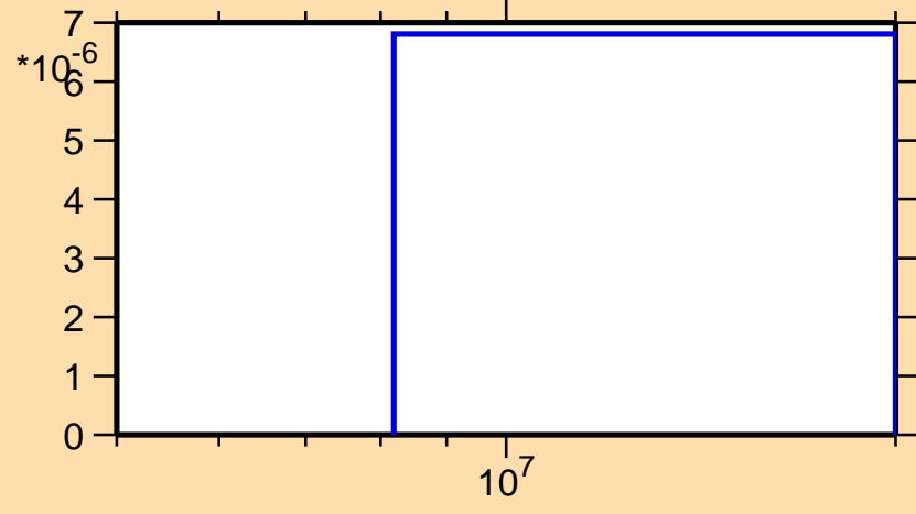
\sigma vs. E for ^{136}\text{Pm}(\text{mt 45})
