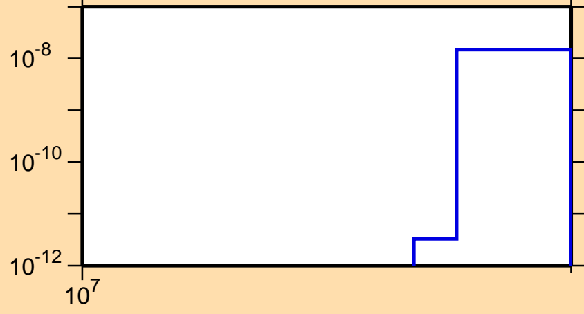
\sigma vs. E for ^{137}\text{Pm}(n,nt)
