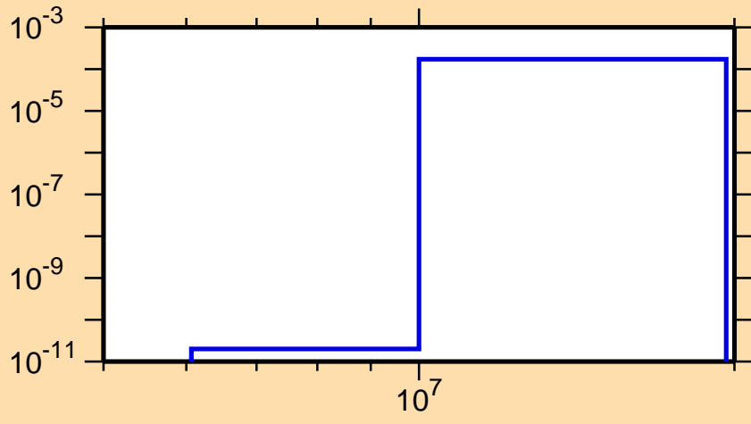
\sigma vs. E for ^{137}\text{Pm}(n,t)
