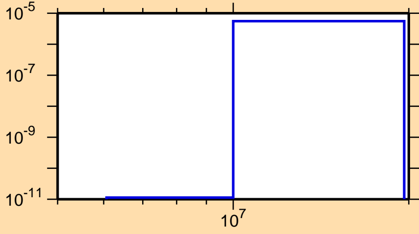
\sigma vs. E for ^{137}\text{Pm}(n,\text{He3})
