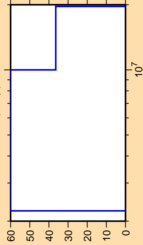
\Delta\sigma/\sigma vs. E for ^{137}\text{Pm}(n,np)
