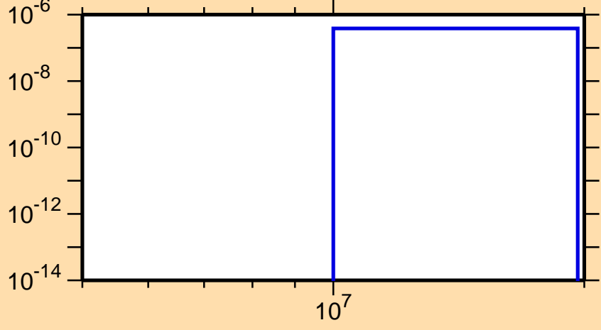
\sigma vs. E for ^{137}\text{Pm}(n,\text{pd})
