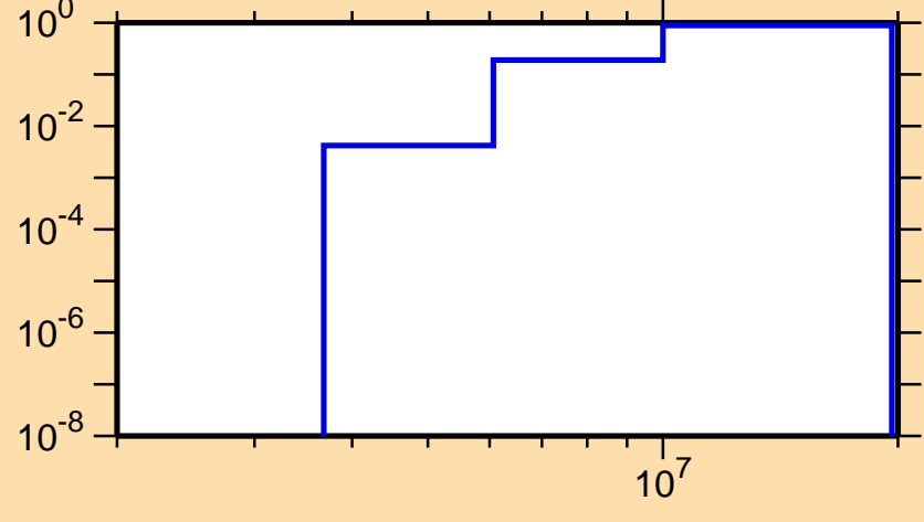
\sigma vs. E for ^{137}\text{Pm}(n,np)
