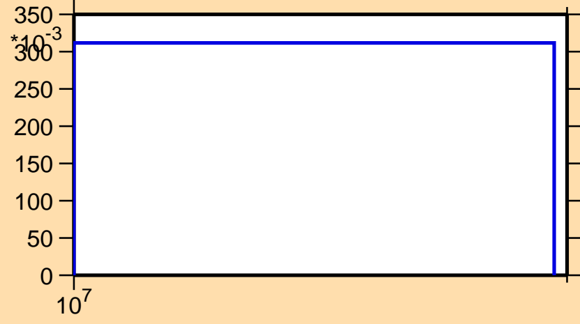
\sigma vs. E for ^{137}\text{Pm}(n,2n)
