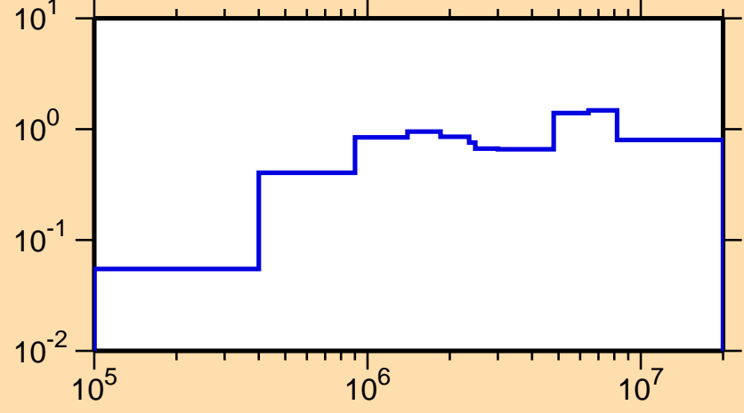
\sigma vs. E for ^{137}\text{Pm}(n,\text{inel.})
