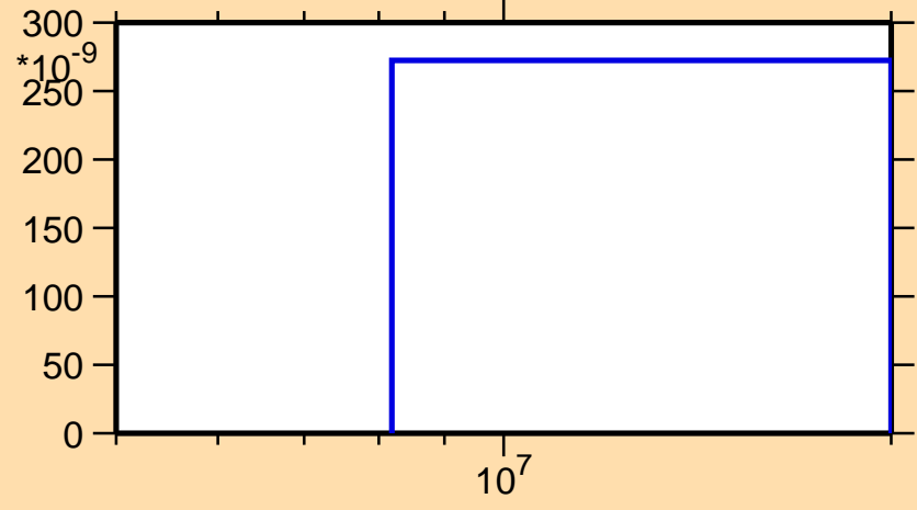
\sigma vs. E for ^{137}\text{Pm}(n,\text{nd})
