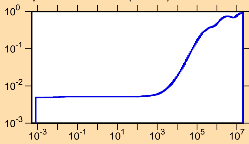
\mu vs. E for ^{138}\text{Pm}(\text{mt251})
