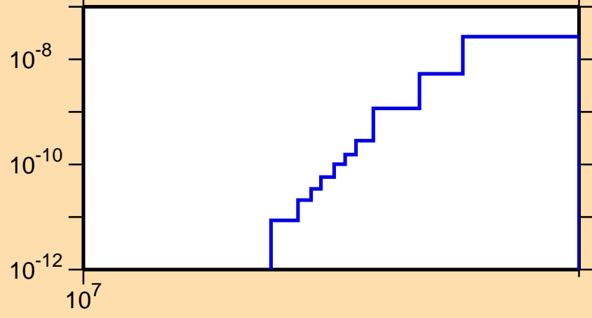
\sigma vs. E for ^{138}\text{Pm}(\text{mt117})
