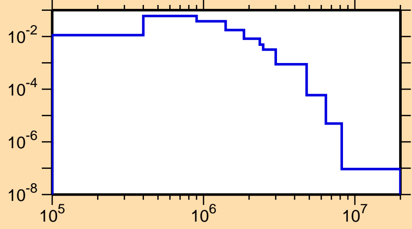
\sigma vs. E for ^{138}\text{Pm}(n,n_4)
