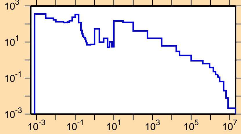
\sigma vs. E for ^{138}\text{Pm}(n,\gamma)
