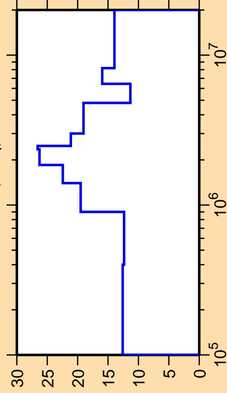
\Delta\sigma/\sigma vs. E for ^{138}\text{Pm}(n,n_4)
