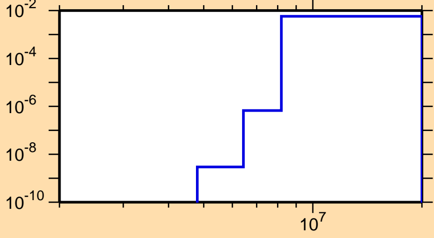
\sigma vs. E for ^{138}\text{Pm}(n,n\alpha)
