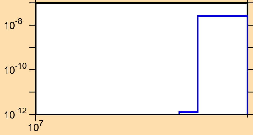
\sigma vs. E for ^{138}\text{Pm}(n,nt)
