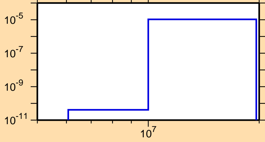
\sigma vs. E for ^{138}\text{Pm}(n,\text{He3})
