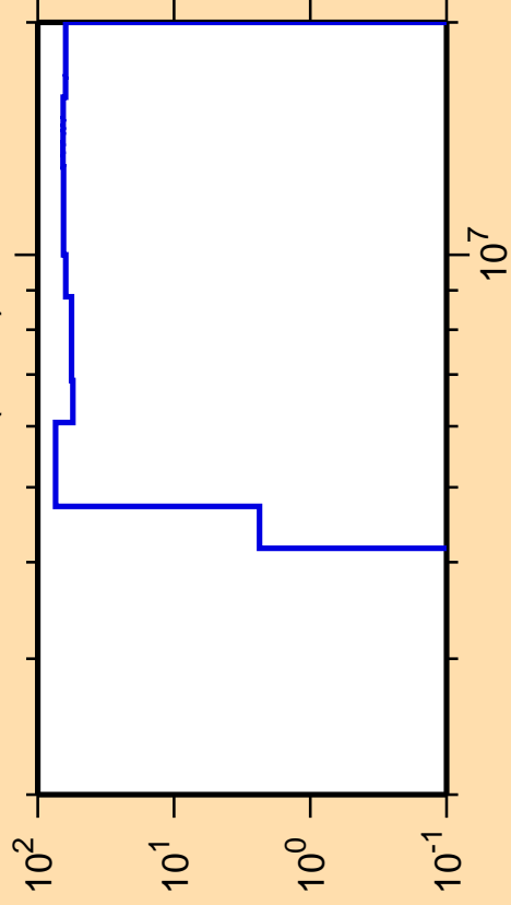
\Delta\sigma/\sigma vs. E for ^{139}\text{Pm}(n,n\alpha)
