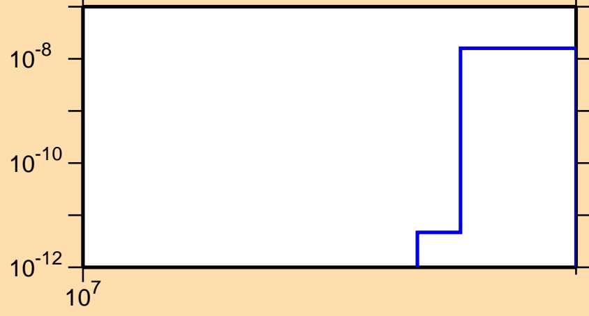
\sigma vs. E for ^{139}\text{Pm}(n,nt)
