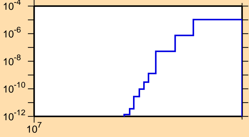
\sigma vs. E for ^{139}\text{Pm}(n,nd)
