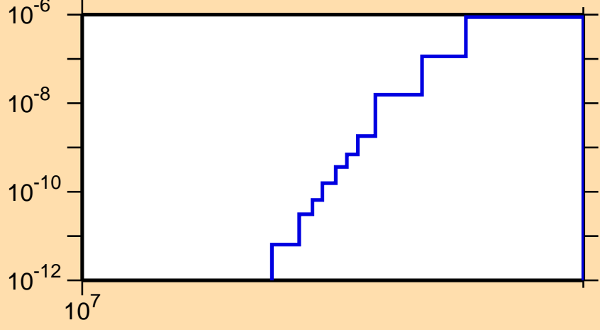
\sigma vs. E for ^{139}\text{Pm}(n,pd)
