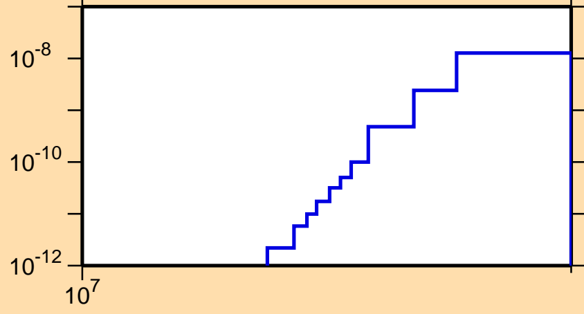
\sigma vs. E for ^{139}\text{Pm}(\text{mt117})
