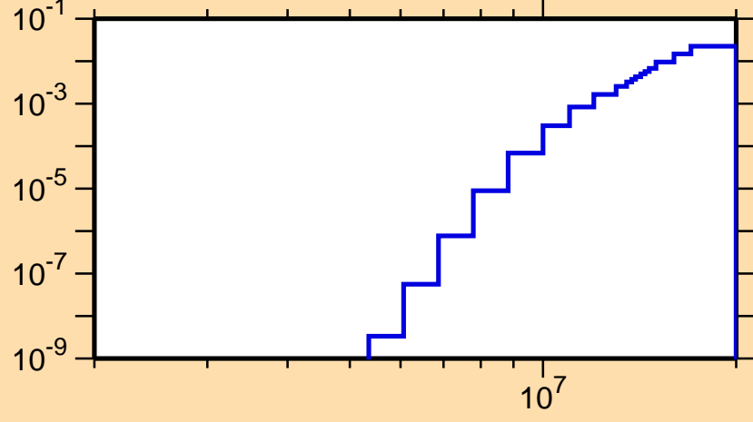
\sigma vs. E for ^{139}\text{Pm}(n,n\alpha)
