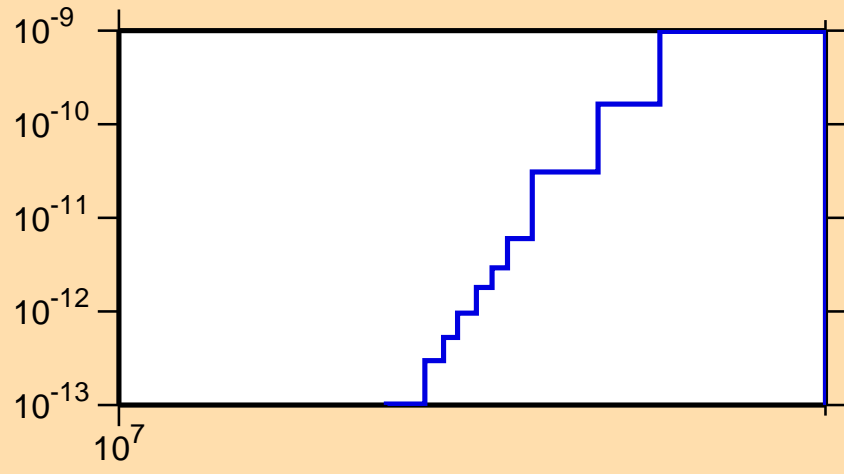
\sigma vs. E for ^{140}\text{Pm}(\text{mt117})
