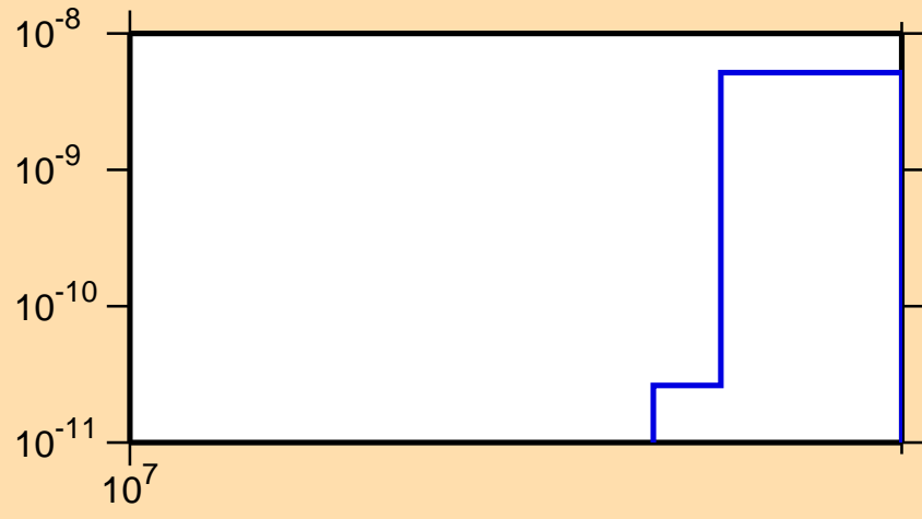
\sigma vs. E for ^{140}\text{Pm}(n,pt)
