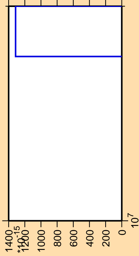
\Delta\sigma/\sigma vs. E for ^{140}\text{Pm}(\text{mt 11})
