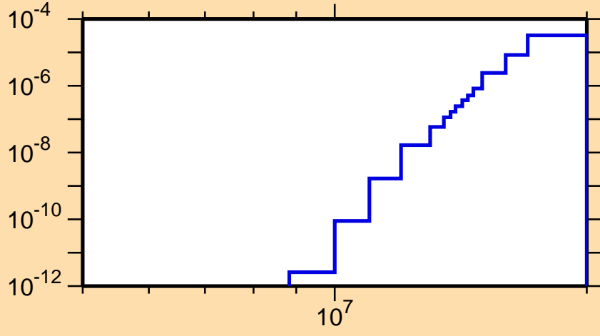
\sigma vs. E for ^{140}\text{Pm}(n,\text{He3})
