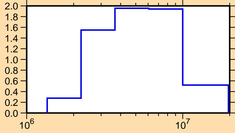
\sigma vs. E for ^{140}\text{Pm}(n,n\text{cont.})
