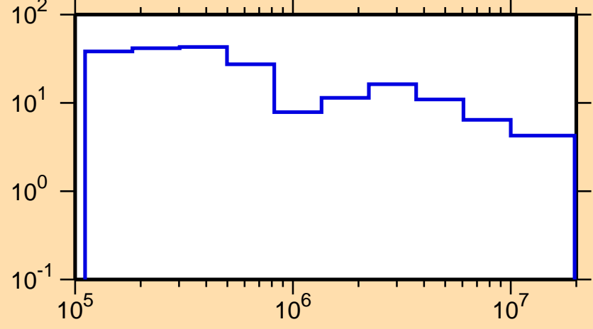
\Delta\sigma/\sigma vs. E for ^{140}\text{Pm}(n,\text{el.})
