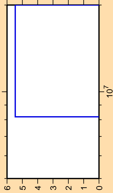
\Delta\sigma/\sigma vs. E for ^{140}\text{Pm}(\text{mt } 34)
