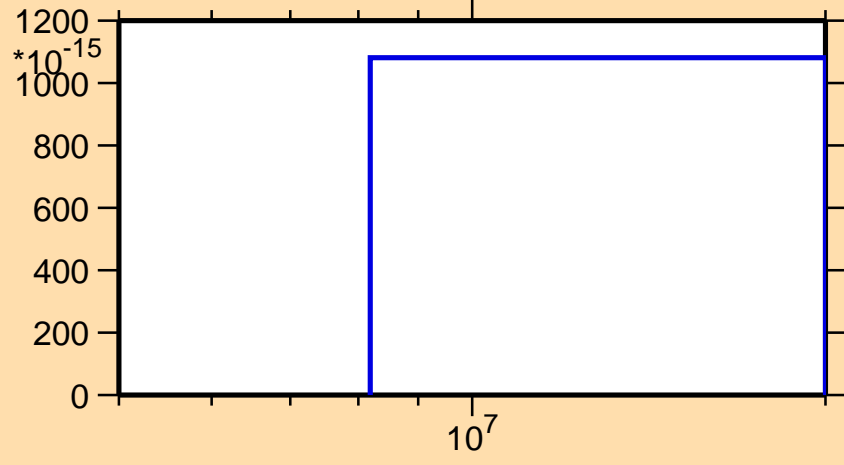
\sigma vs. E for ^{140}\text{Pm}(\text{mt } 34)
