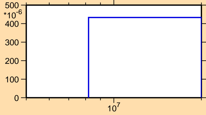
\sigma vs. E for ^{140}\text{Pm}(n,2np)
