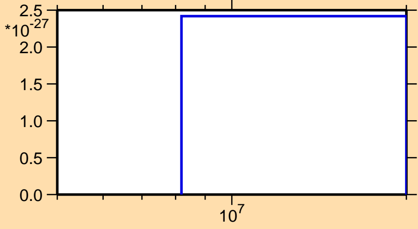
\sigma vs. E for ^{140}\text{Pm}(\text{mt 11})
