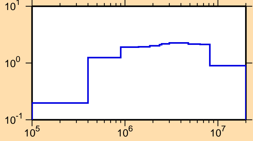
\sigma vs. E for ^{140}\text{Pm}(n,\text{inel.})
