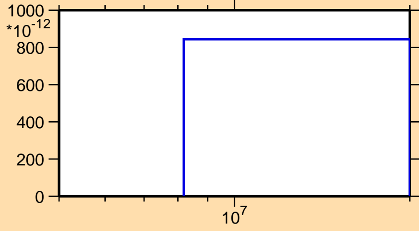
\sigma vs. E for ^{140}\text{Pm}(\text{mt 45})
