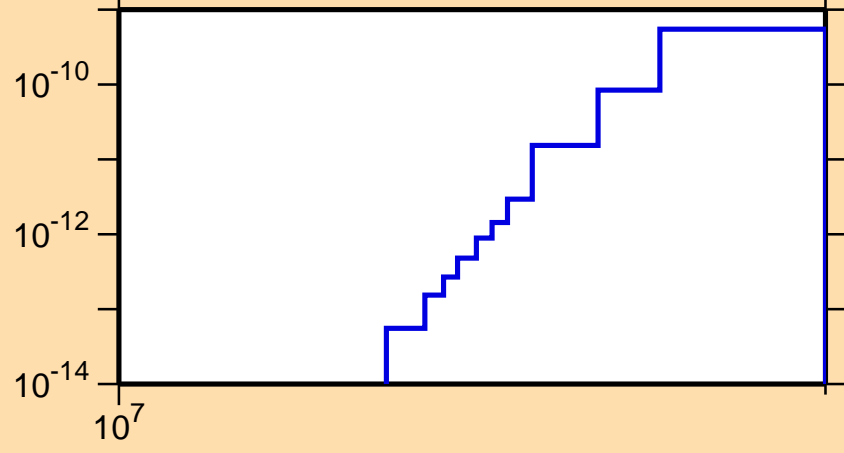
\sigma vs. E for ^{140}\text{Pm}(\text{mt117})
