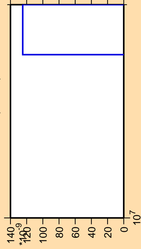
\Delta\sigma/\sigma vs. E for ^{140}\text{Pm} (mt 11)
