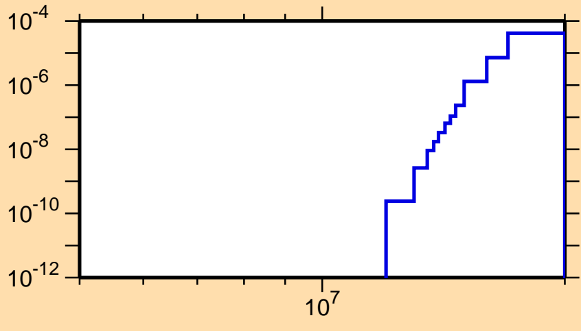
\sigma vs. E for ^{140}\text{Pm}(n,\text{nd})
