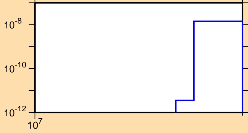
\sigma vs. E for ^{140}\text{Pm}(n,nt)
