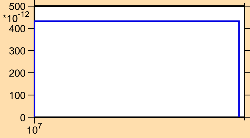
\sigma vs. E for ^{140}\text{Pm}(n,pd)
