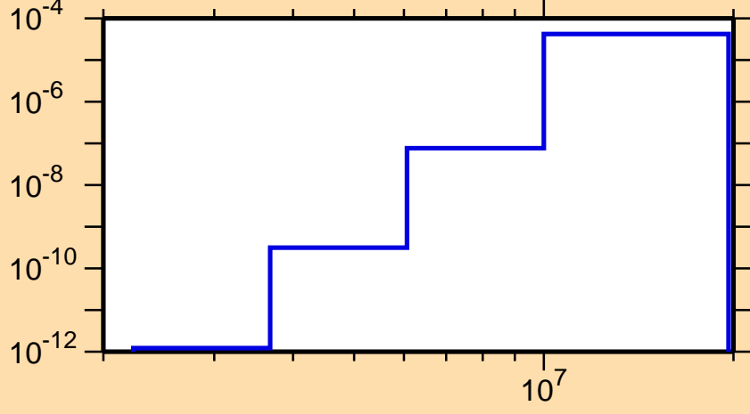
\sigma vs. E for ^{140}\text{Pm}(n,p\alpha)
