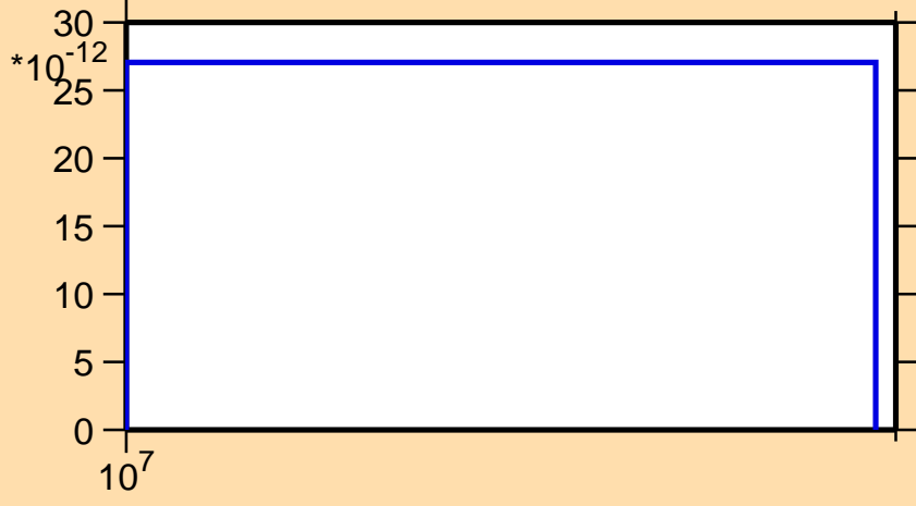
\sigma vs. E for ^{140}\text{Pm}(n,pt)
