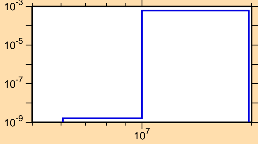
\sigma vs. E for ^{140}\text{Pm}(n,t)
