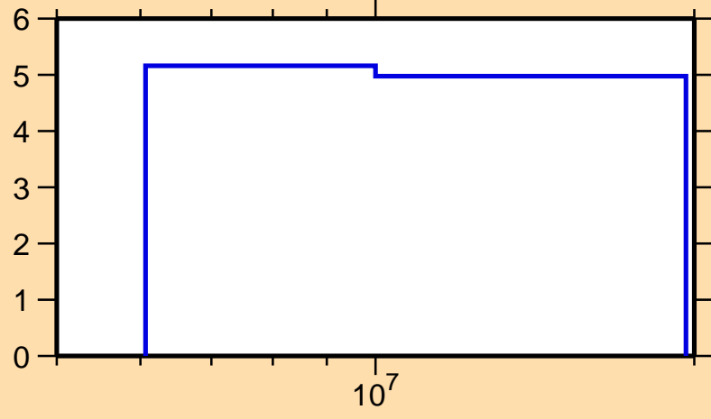
\Delta\sigma/\sigma vs. E for ^{140}\text{Pm}(n,\text{el.})
