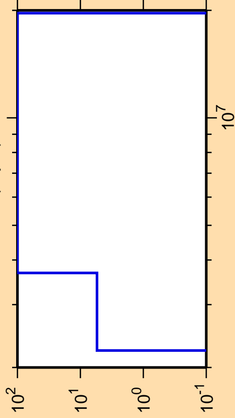
\Delta\sigma/\sigma vs. E for ^{140}\text{Pm}(n,p\alpha)
