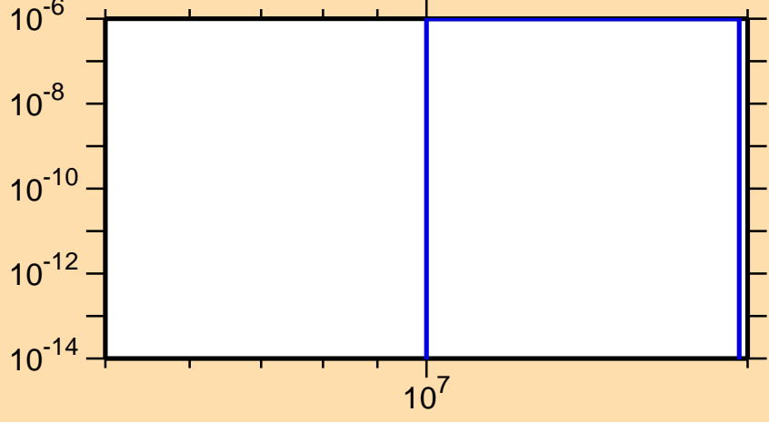
\sigma vs. E for ^{140}\text{Pm}(n,\text{nd})
