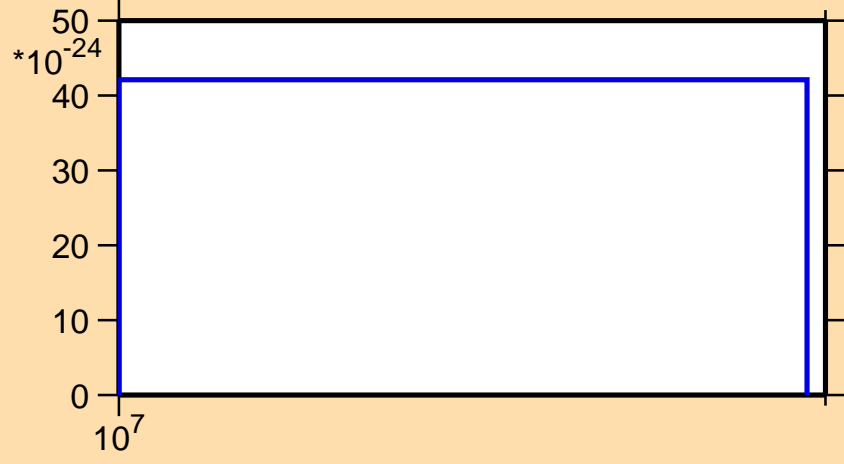
\sigma vs. E for ^{140}\text{Pm} (mt 11)
