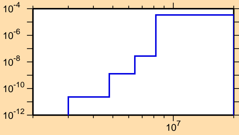
\sigma vs. E for ^{140}\text{Pm}(n,p\alpha)
