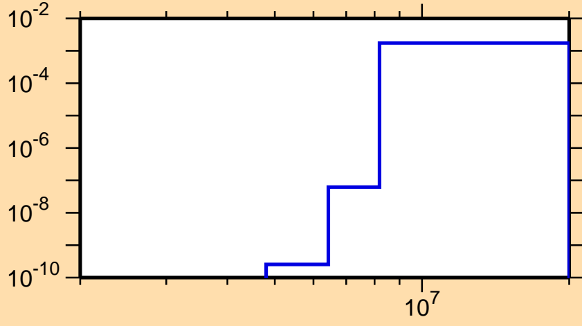
\sigma vs. E for ^{140}\text{Pm}(n,n\alpha)
