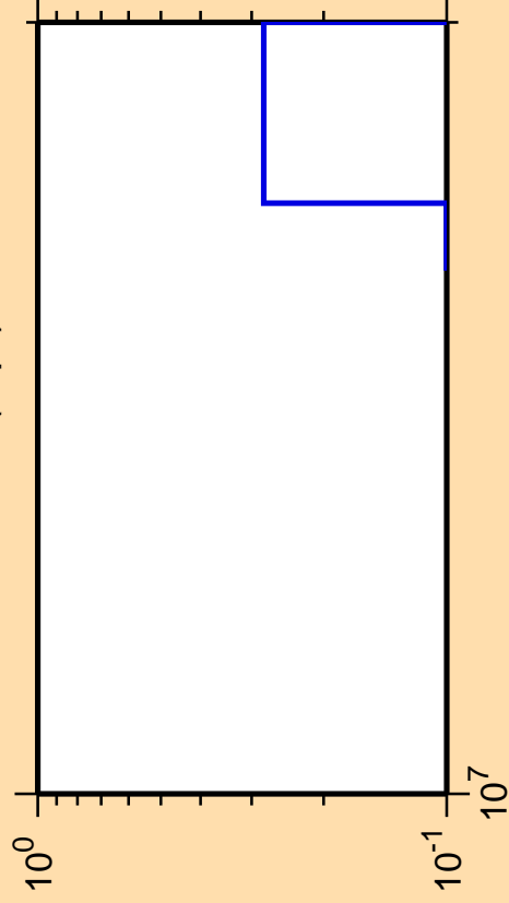
\Delta\sigma/\sigma vs. E for ^{141}\text{Pm}(n,pt)
