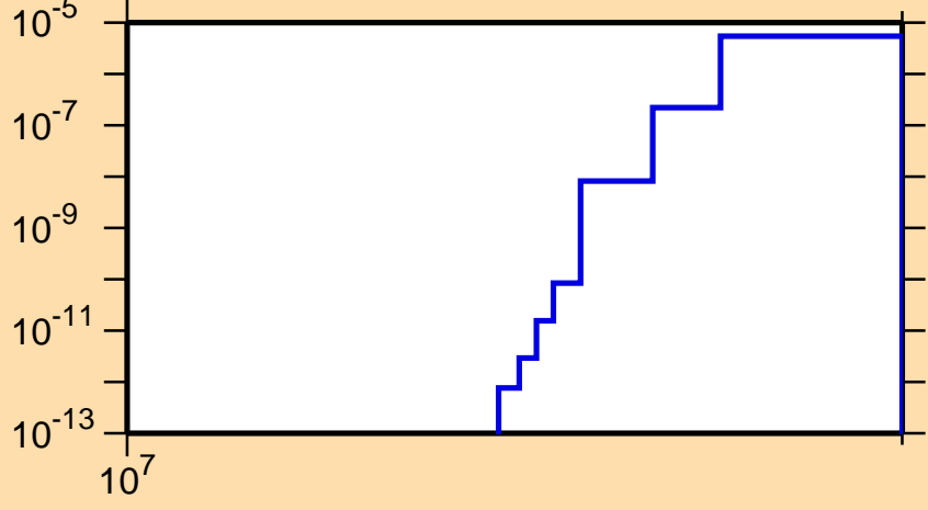
\sigma vs. E for ^{141}\text{Pm}(n,nd)
