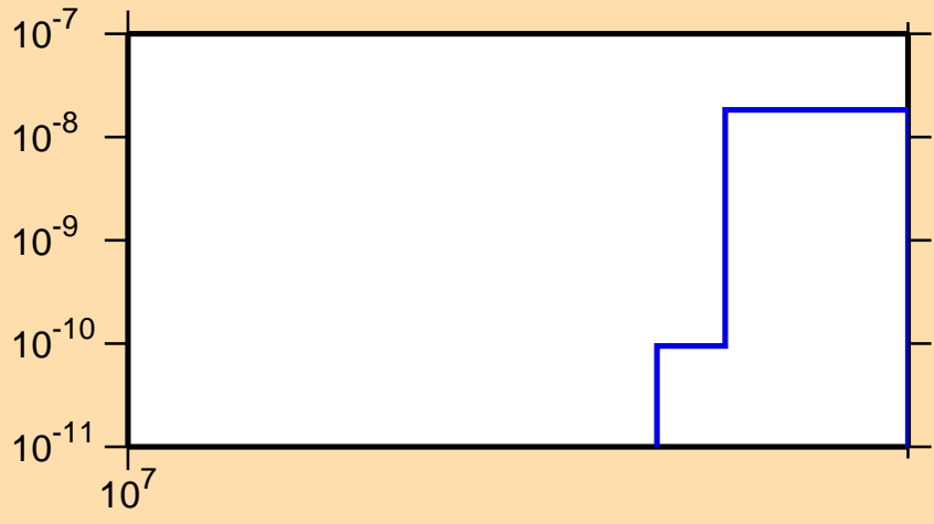
\sigma vs. E for ^{141}\text{Pm}(n,2n\alpha)
