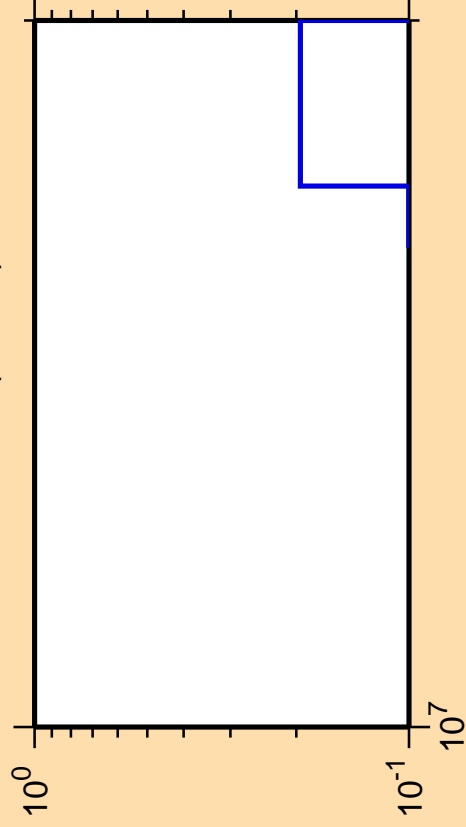
\Delta\sigma/\sigma vs. E for ^{141}\text{Pm} (mt 34)
