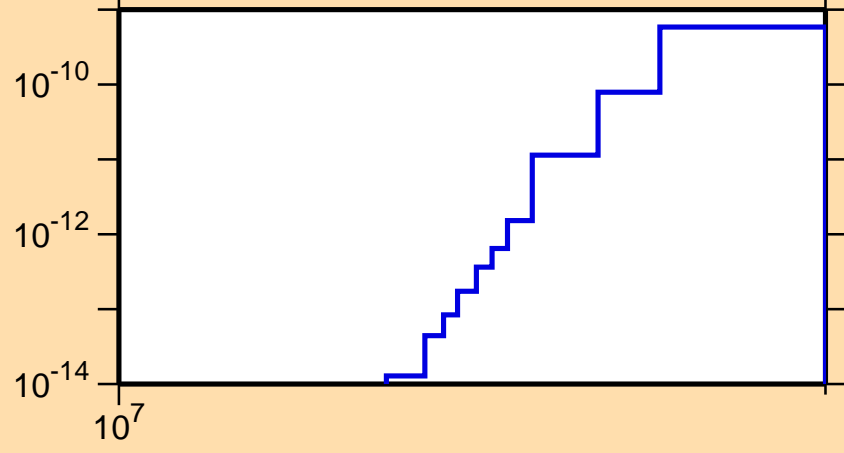
\sigma vs. E for ^{141}\text{Pm}(\text{mt117})
