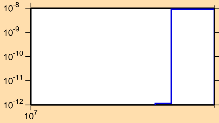
\sigma vs. E for ^{141}\text{Pm}(n,nt)
